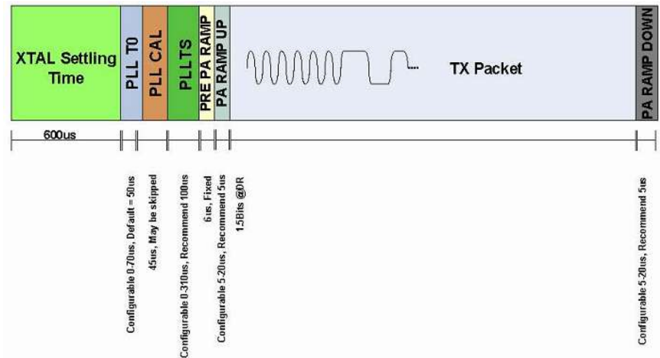
Figure 6. TX Timing
