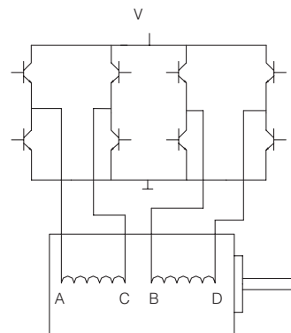
2 phase stepping motor with bipolar driver
