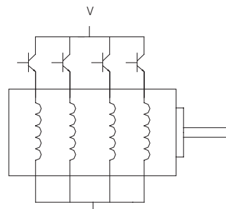
4 phase stepping motor with unipolar driver
