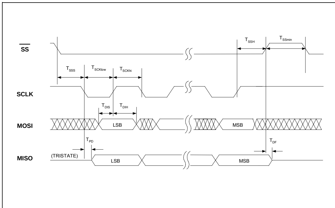
Figure 12.8: SPI Operation
