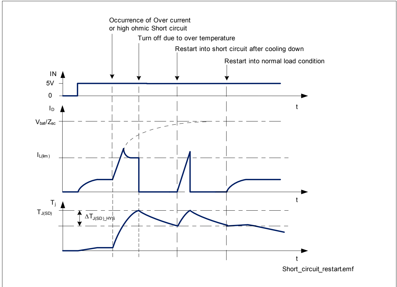
Figure 15 Short circuit protection via current limitation and over temperature switch off with auto-restart
