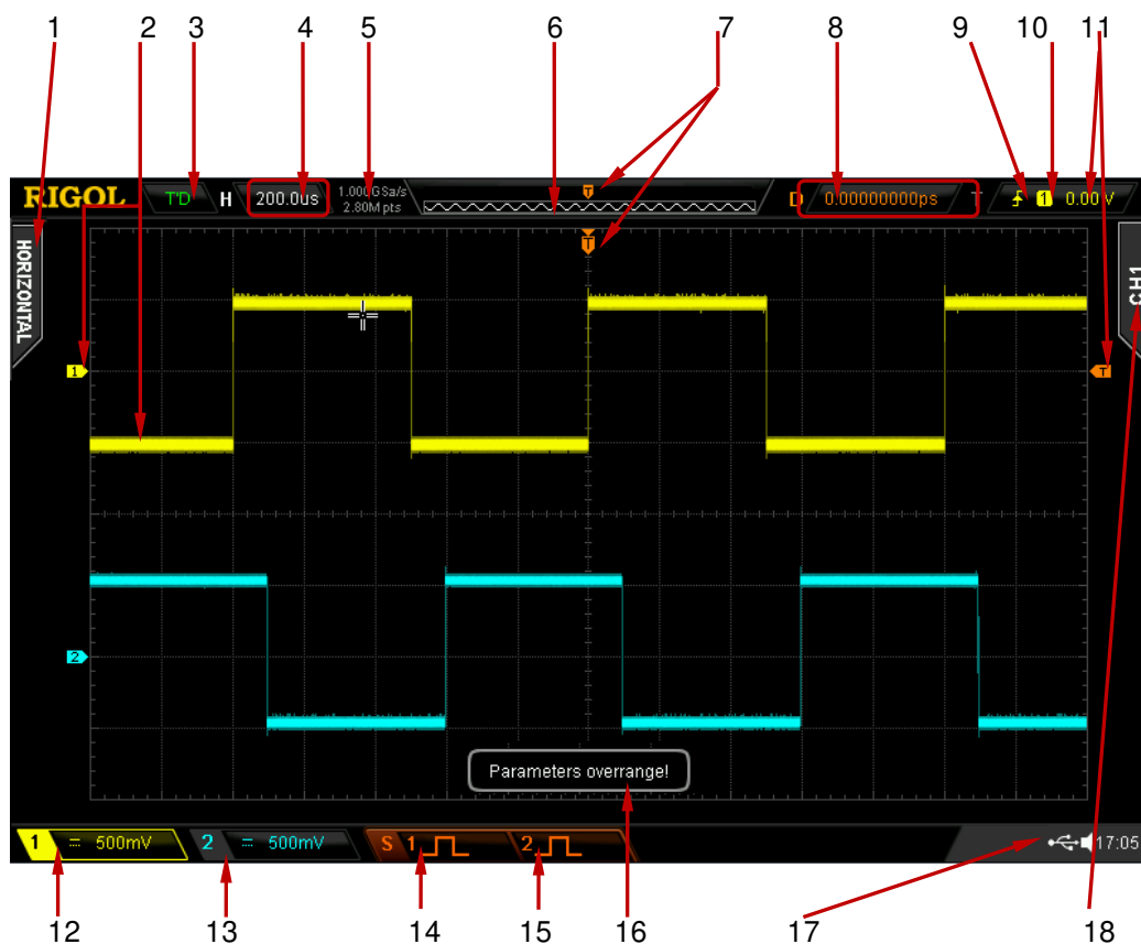
Figure 1-11 User Interface
