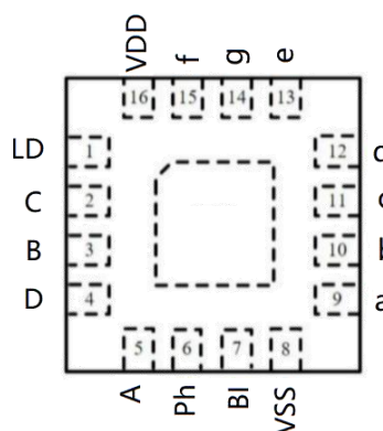
QFN-16 3*3
