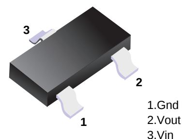
■ Simplified outline(SOT23-3L)
