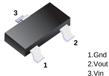
■ Simplified outline(SOT-23)
