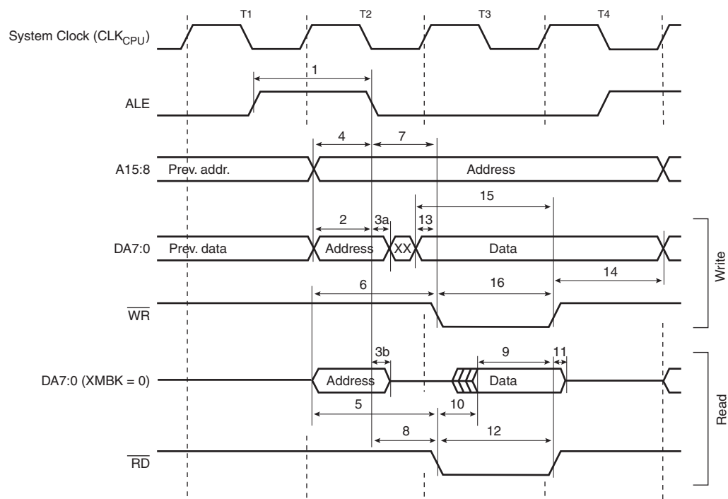
Figure 157. External Memory Timing (SRWn1 = 0, SRWn0 = 0)
