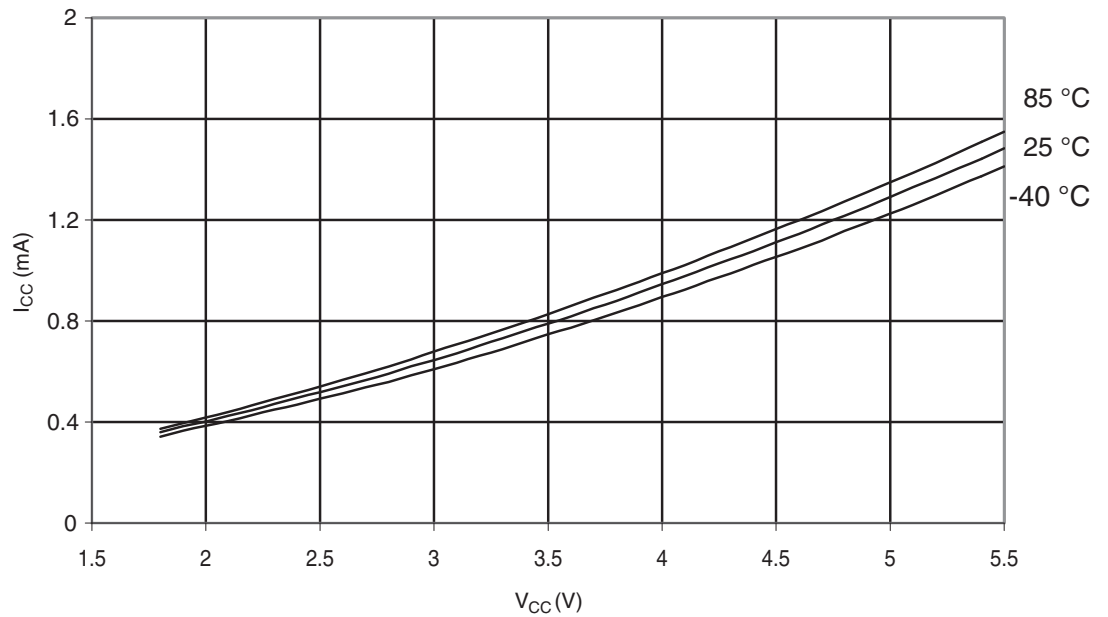
Figure 30-292. ATmega328: Idle Supply Current vs. V_{CC} (Internal RC Oscillator, 8MHz)
