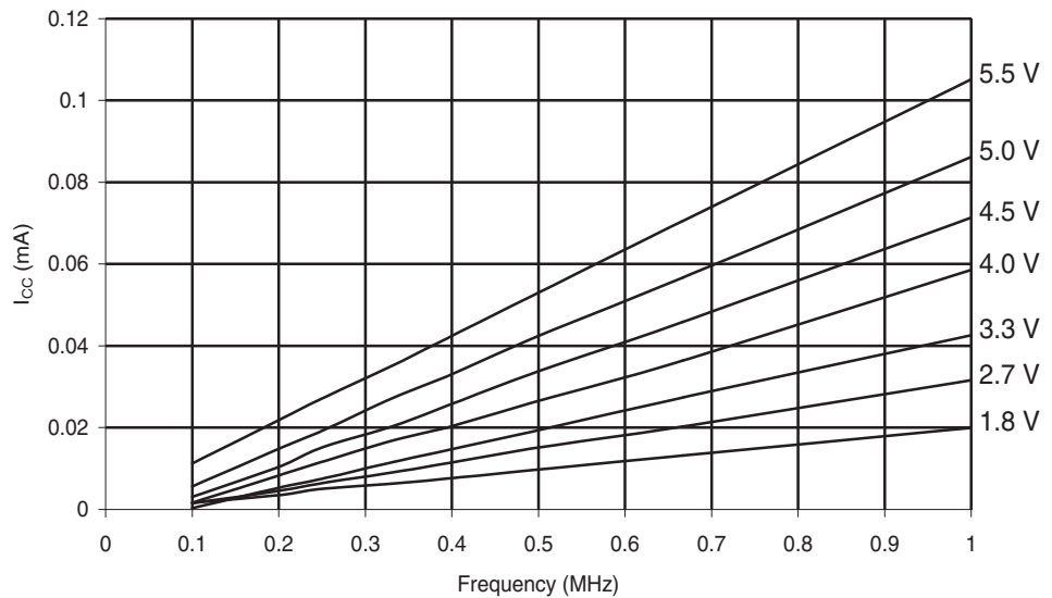
Figure 30-233. ATmega168A: Reset Supply Current vs. Low Frequency (0.1 - 1.0MHz)
