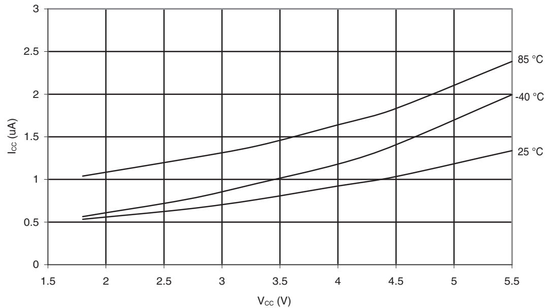
Figure 30-154. ATmega88PA: Power-Save Supply Current vs. V_{CC} (Watchdog Timer Disabled and 32kHz Crystal Oscillator Running)
