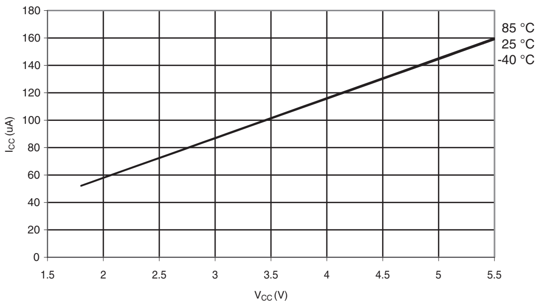
Figure 30-324. ATmega328: AREF External Reference Current vs. V_{CC}
