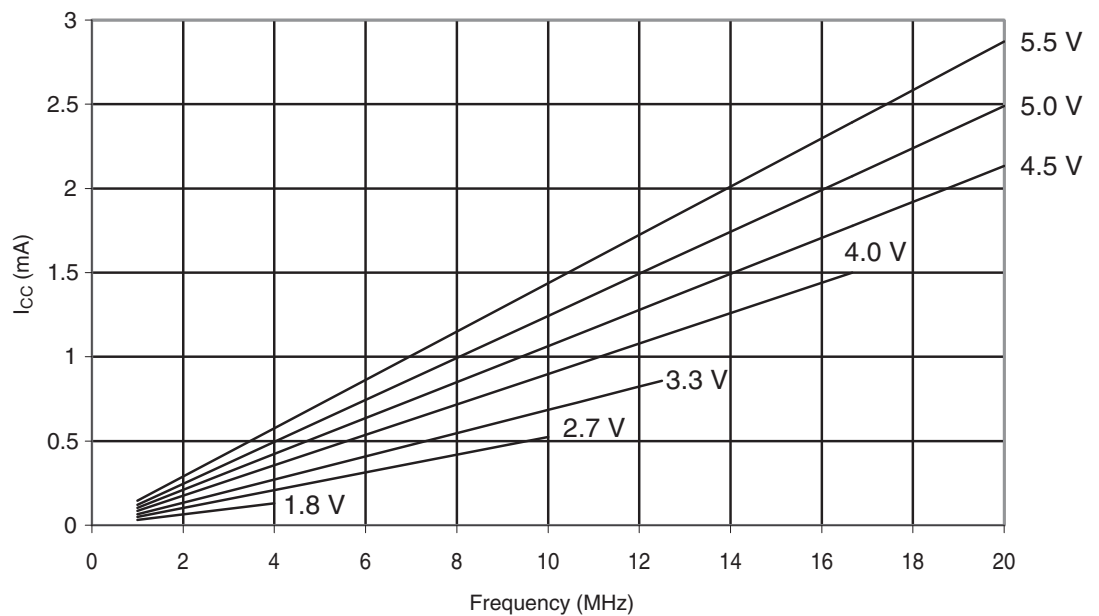
Figure 30-375. ATmega328P: Reset Supply Current vs. Frequency (1 - 20MHz)
