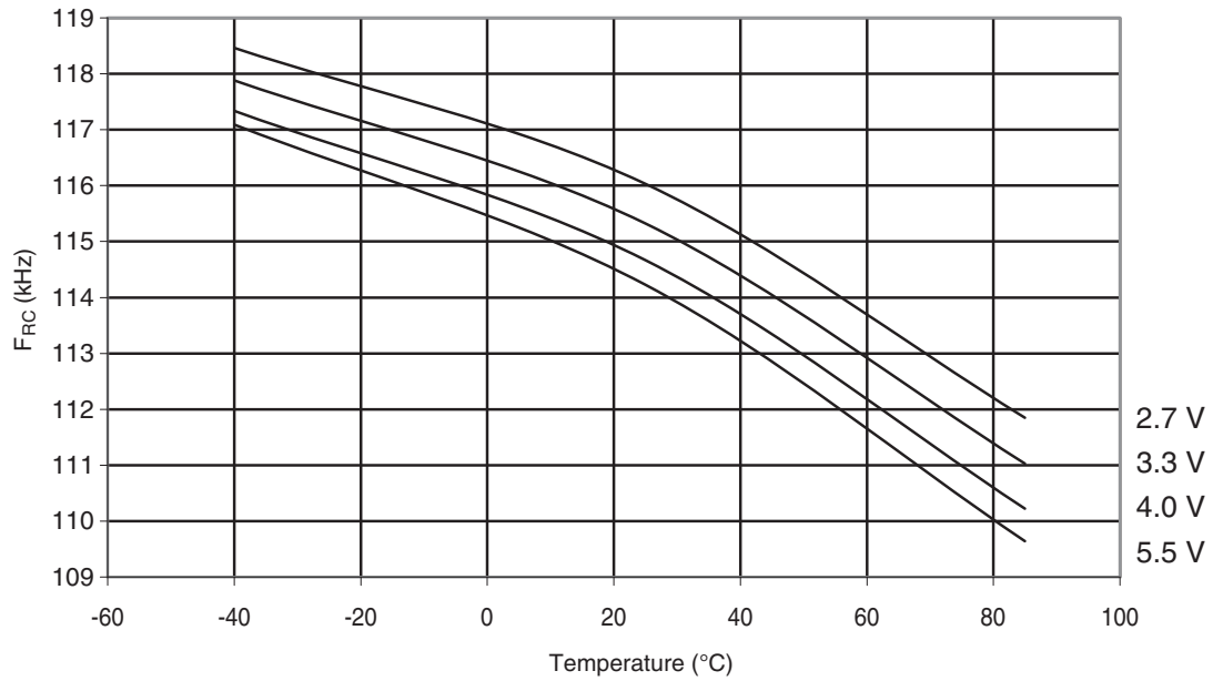
Figure 30-317. ATmega328: Watchdog Oscillator Frequency vs. Temperature
