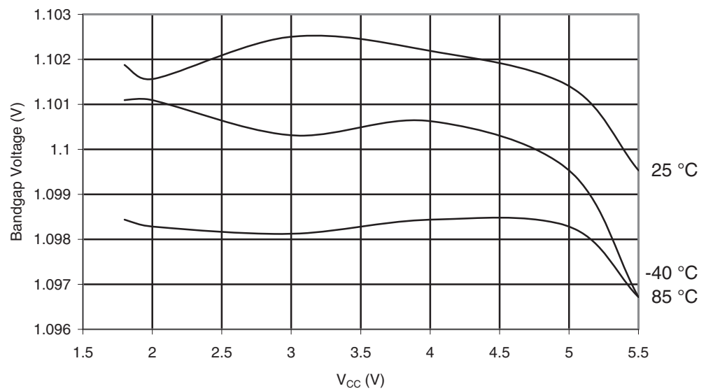
Figure 30-175. ATmega88PA: Bandgap Voltage vs. V_{CC}
