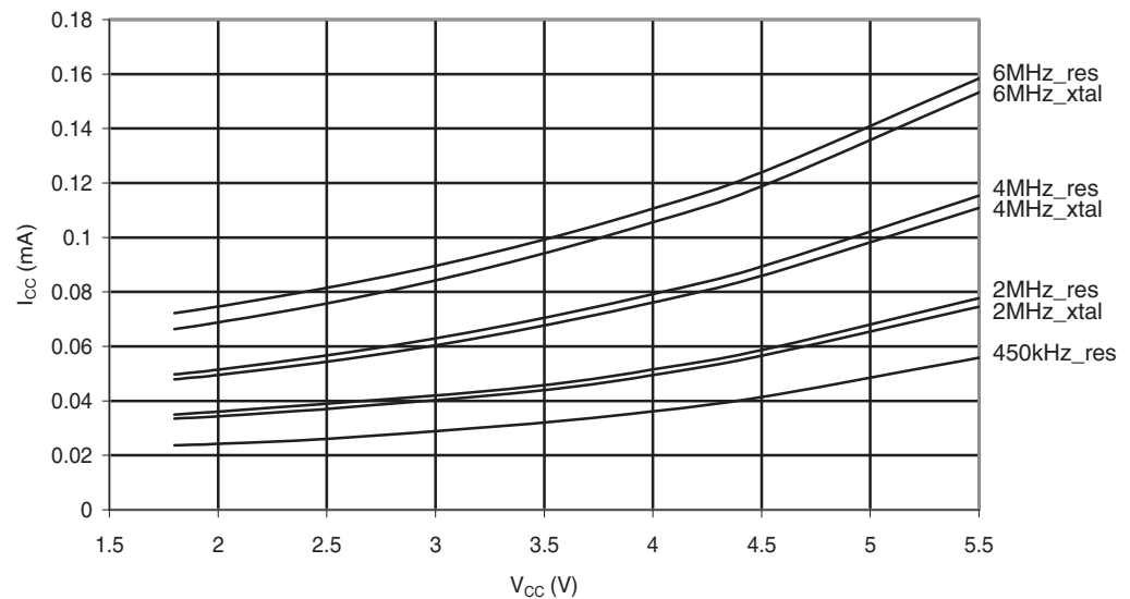
Figure 30-108. ATmega88A: Standby Supply Current vs. V_{CC} (Watchdog Timer Disabled)
