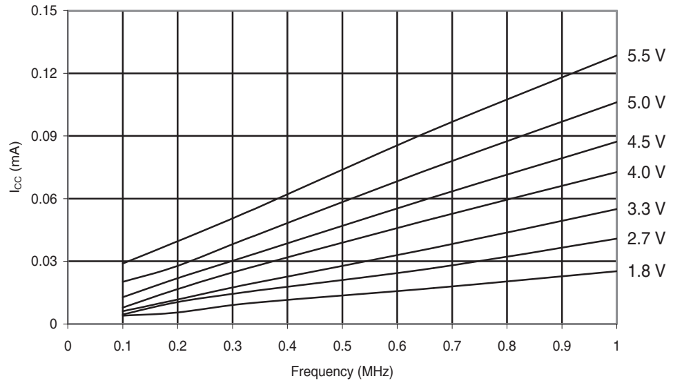
Figure 30-100. ATmega88A: Idle Supply Current vs. Low Frequency (0.1-1.0MHz)
