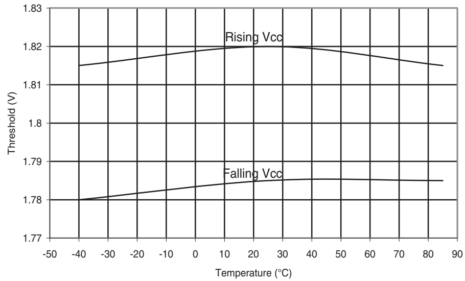
Figure 30-125. ATmega88A: BOD Thresholds vs. Temperature (BODLEVEL is 1.8 V)
