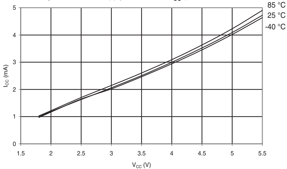
Figure 30-99. ATmega88A: Active Supply Current vs. V_{CC} (Internal RC Oscillator, 8MHz)
