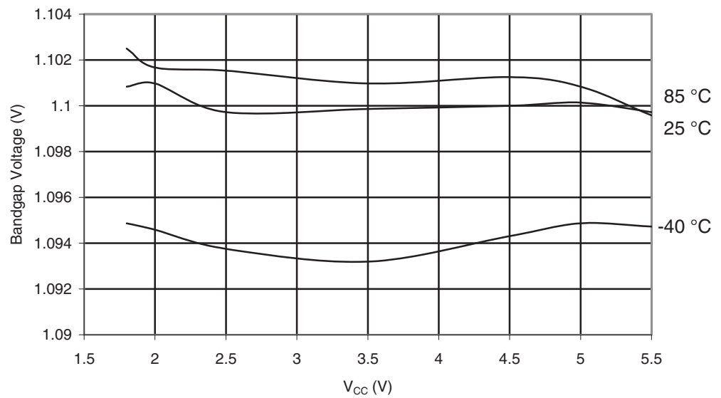
Figure 30-81. ATmega48PA: Bandgap Voltage vs. V_{CC}
