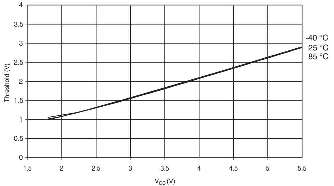
Figure 30-354. ATmega328P: I/O Pin Input Threshold Voltage vs. V_{CC} ( V_{IH} , I/O Pin read as '1')
