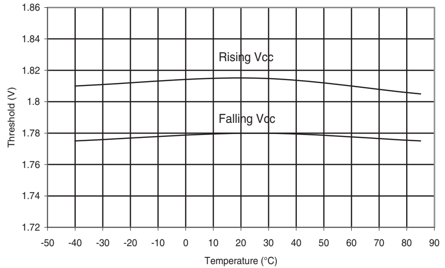
Figure 30-219. ATmega168A: BOD Thresholds vs. Temperature (BODLEVEL is 1.8 V)
