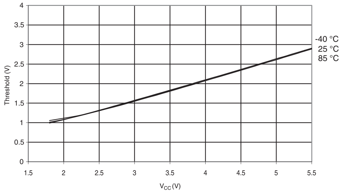
Figure 30-307. ATmega328: I/O Pin Input Threshold Voltage vs. V_{CC} ( V_{IH} , I/O Pin read as '1')
