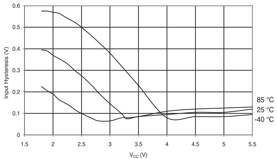
Figure 30-171. ATmega88PA: Reset Pin Input Hysteresis vs. V_{CC}
