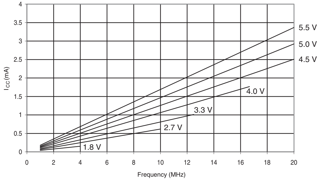
Figure 30-289. ATmega328: Idle Supply Current vs. Frequency (1-20MHz)
