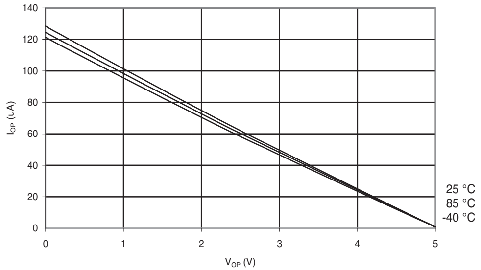
Figure 30-64. ATmega48PA: I/O Pin Pull-up Resistor Current vs. Input Voltage ( V_{CC} = 5\text{ V} )
