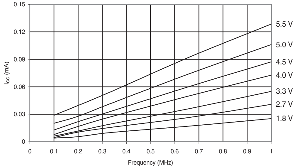
Figure 30-147. ATmega88PA: Idle Supply Current vs. Low Frequency (0.1-1.0MHz)
