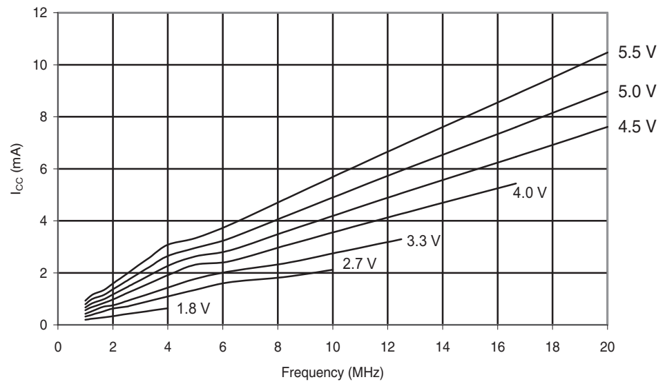
Figure 30-143. ATmega88PA: Active Supply Current vs. Frequency (1 - 20MHz)
