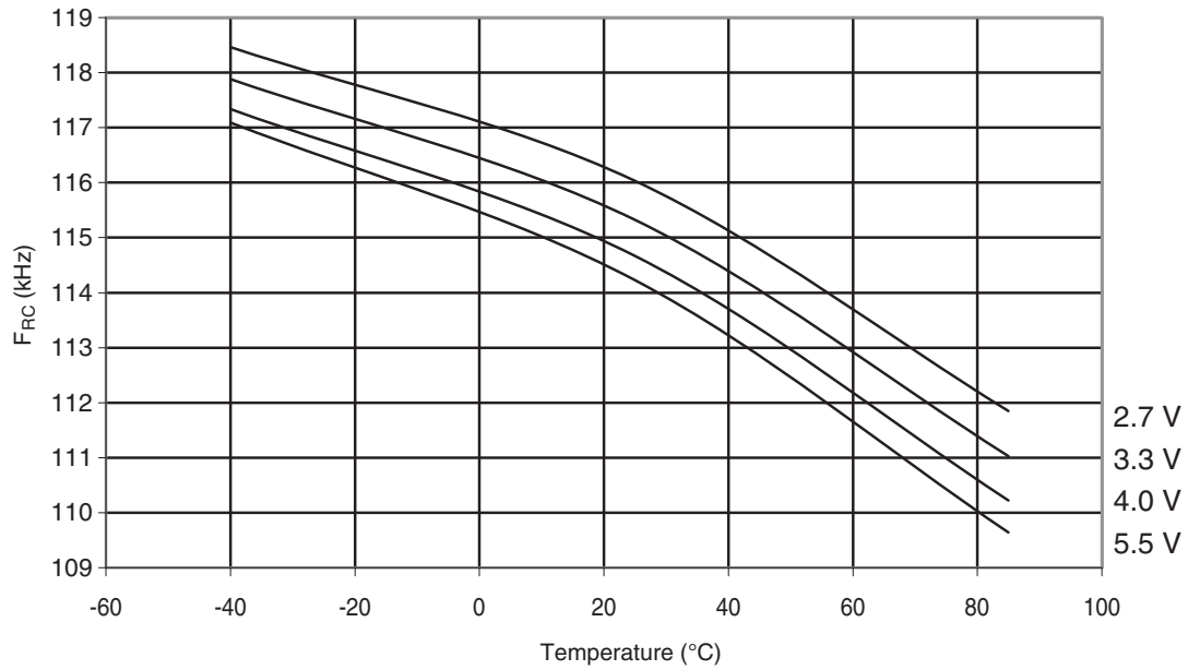
Figure 30-364. ATmega328P: Watchdog Oscillator Frequency vs. Temperature
