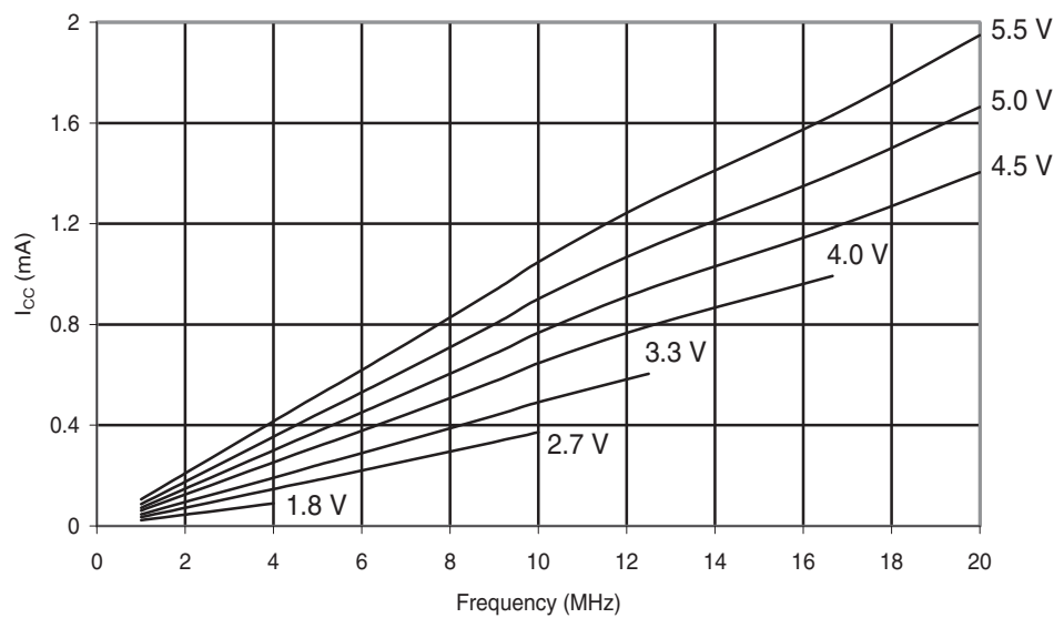
Figure 30-187. ATmega88PA: Reset Supply Current vs. Frequency (1 - 20MHz)
