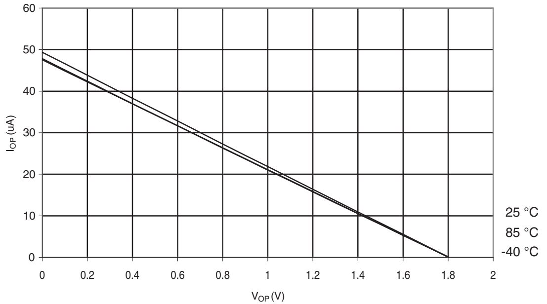
Figure 30-344. ATmega328P: I/O Pin Pull-up Resistor Current vs. Input Voltage ( V_{CC} = 1.8\text{ V} )
