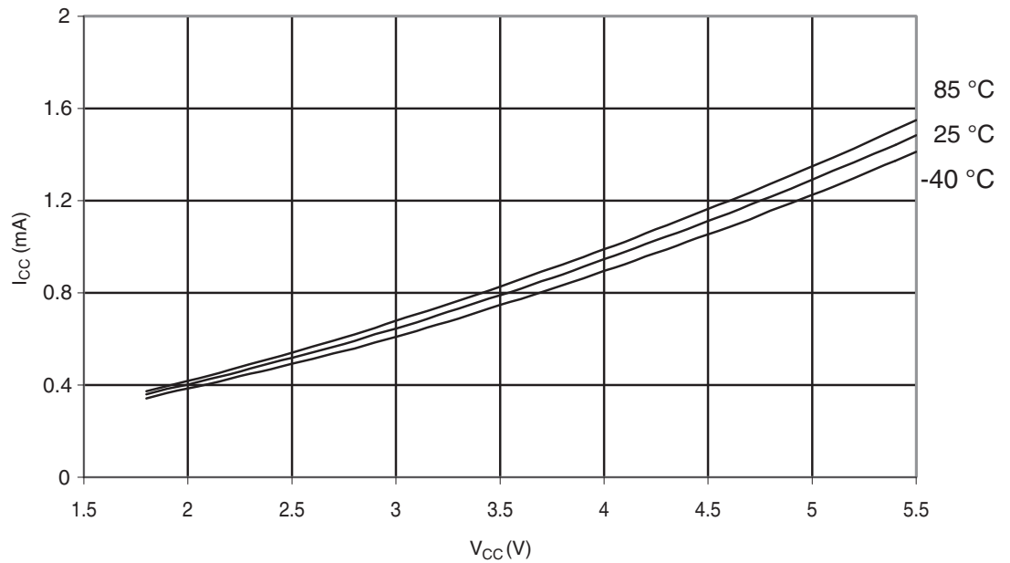
Figure 30-339. ATmega328P: Idle Supply Current vs. V_{CC} (Internal RC Oscillator, 8MHz)
