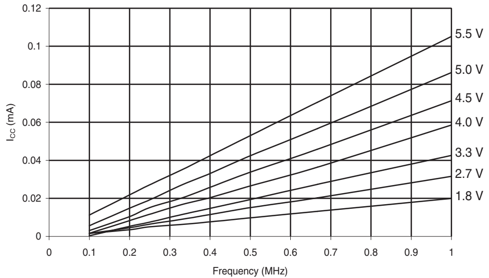
Figure 30-280. ATmega168PA: Reset Supply Current vs. Low Frequency (0.1 - 1.0MHz)
