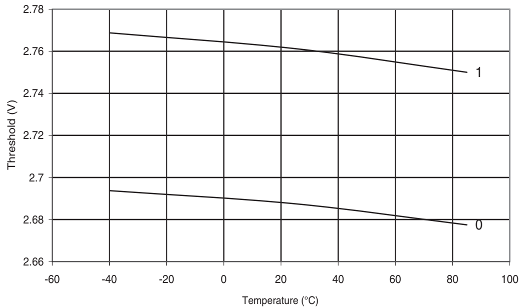
Figure 30-314. ATmega328: BOD Thresholds vs. Temperature (BODLEVEL is 2.7 V)
