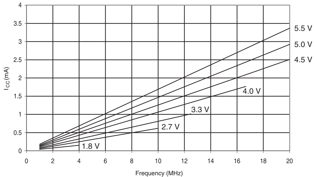
Figure 30-336. ATmega328P: Idle Supply Current vs. Frequency (1-20MHz)
