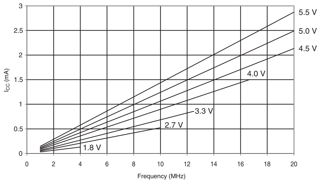
Figure 30-328. ATmega328: Reset Supply Current vs. Frequency (1 - 20MHz)
