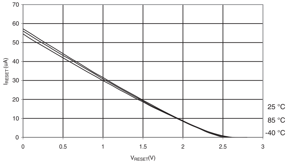
Figure 30-348. ATmega328P: Reset Pull-up Resistor Current vs. Reset Pin Voltage ( V_{CC} = 2.7\text{ V} )
