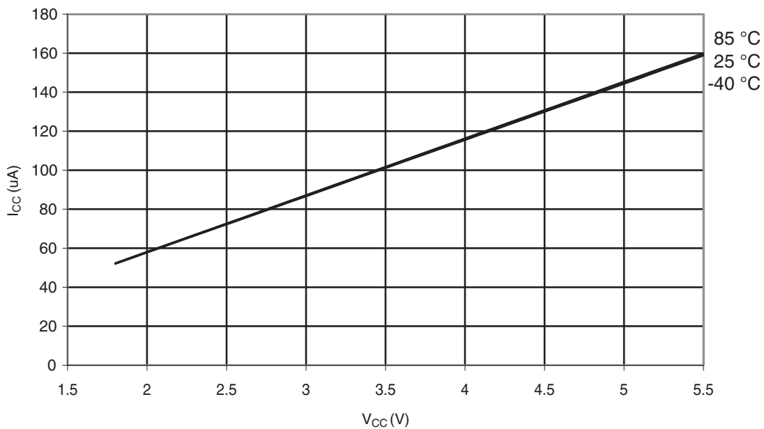
Figure 30-371. ATmega328P: AREF External Reference Current vs. V_{CC}
