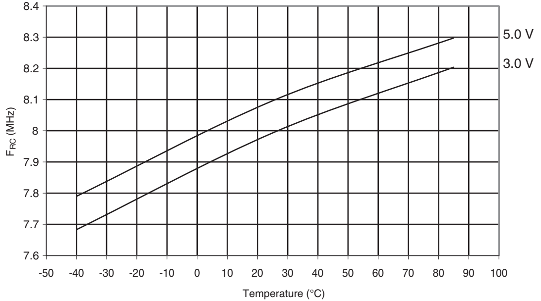
Figure 30-320. ATmega328: Calibrated 8MHz RC Oscillator Frequency vs. Temperature
