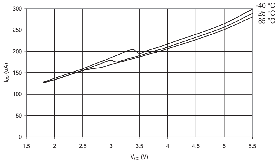
Figure 30-181. ATmega88PA: ADC Current vs. V_{CC} (AREF = AV_{CC} )
