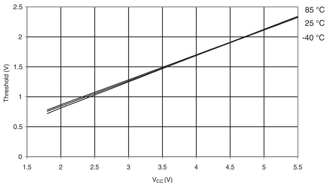
Figure 30-358. ATmega328P: Reset Input Threshold Voltage vs. V_{CC} ( V_{IL} , I/O Pin read as '0')
