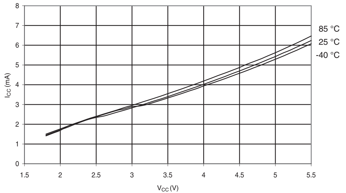
Figure 30-334. ATmega328P: Active Supply Current vs. V_{CC} (Internal RC Oscillator, 8MHz)
