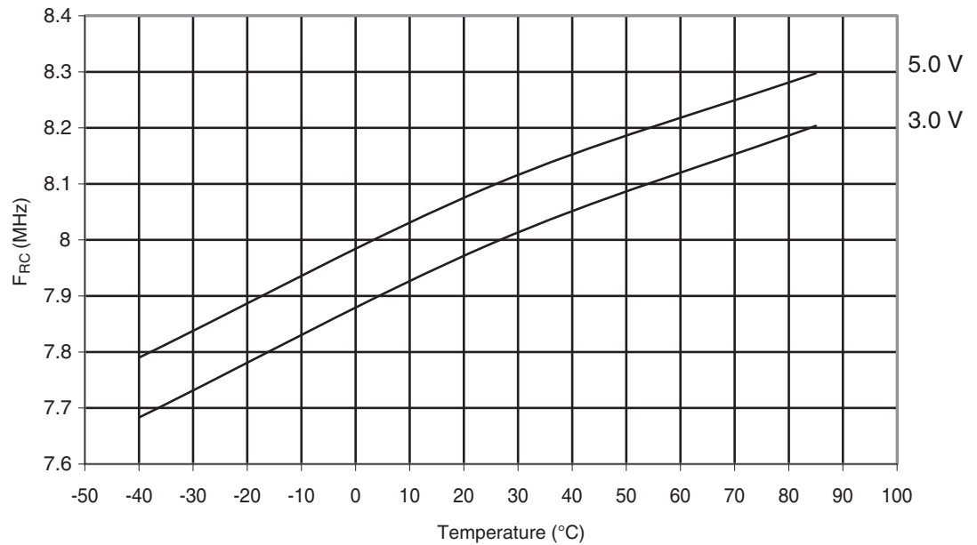
Figure 30-367. ATmega328P: Calibrated 8MHz RC Oscillator Frequency vs. Temperature
