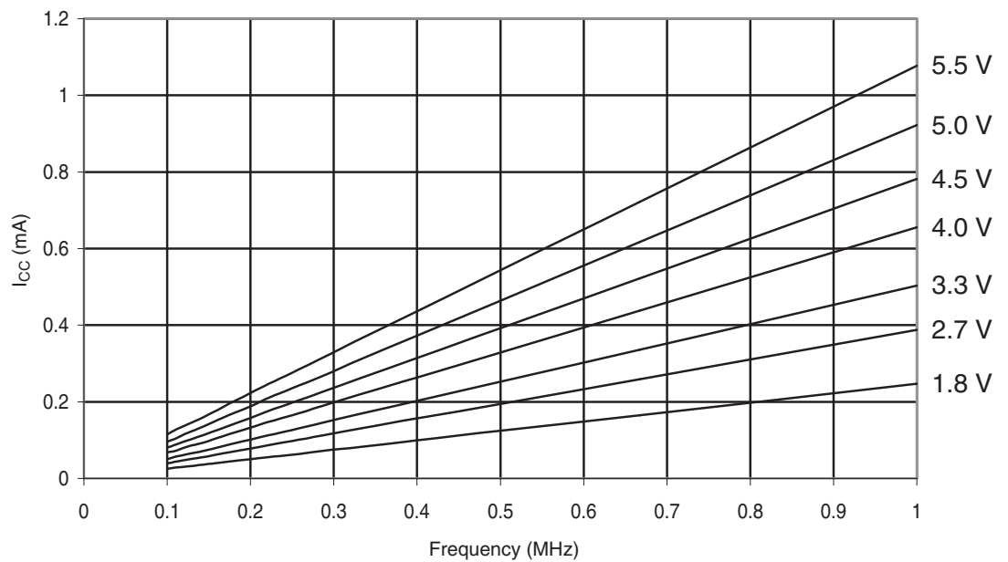
Figure 30-330. ATmega328P: Active Supply Current vs. Low Frequency (0.1-1.0MHz)
