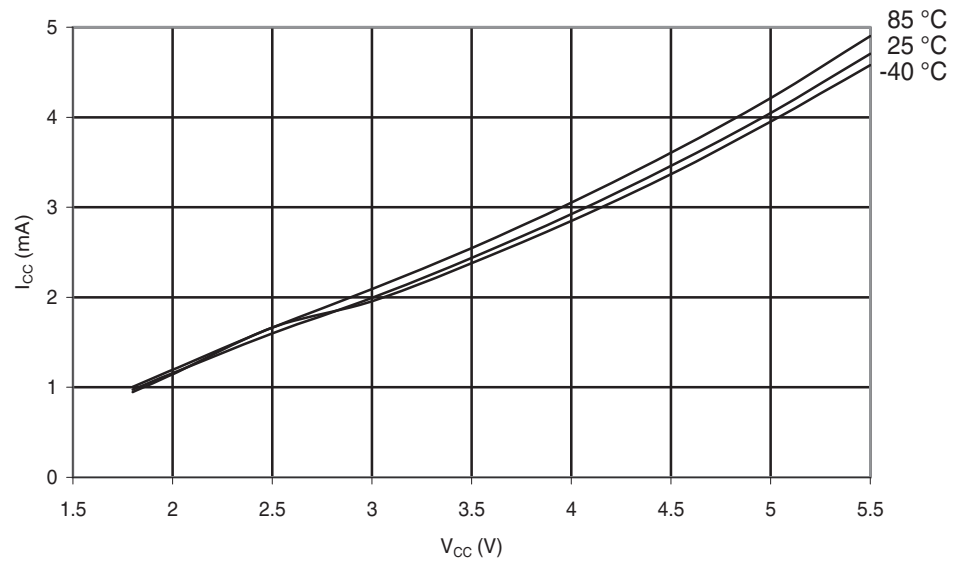
Figure 30-5. ATmega48A: Active Supply Current vs. V_{CC} (Internal RC Oscillator, 8MHz)
