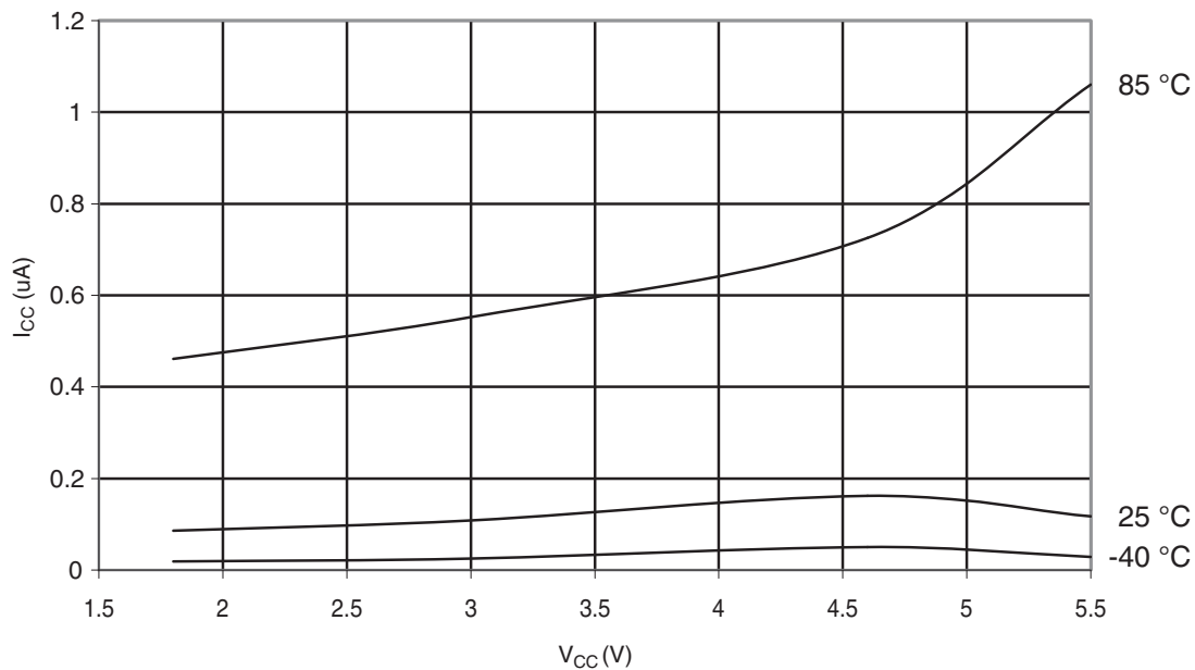
Figure 30-340. ATmega328P: Power-Down Supply Current vs. V_{CC} (Watchdog Timer Disabled)
