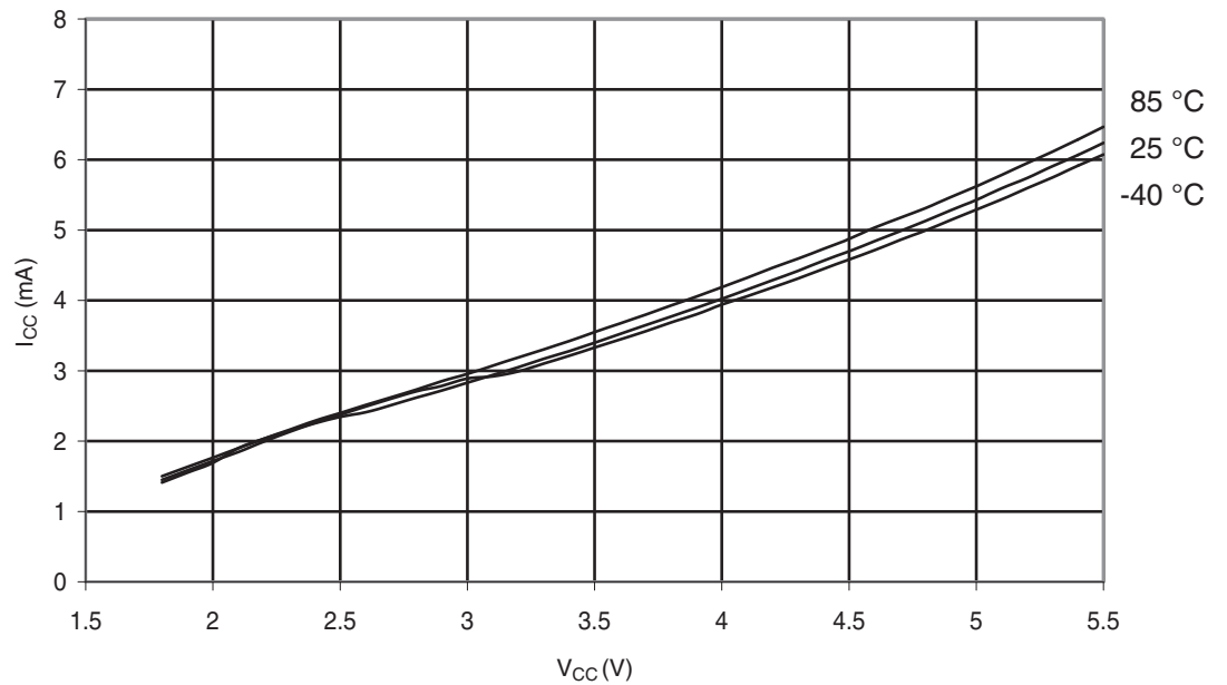
Figure 30-287. ATmega328: Active Supply Current vs. V_{CC} (Internal RC Oscillator, 8MHz)
