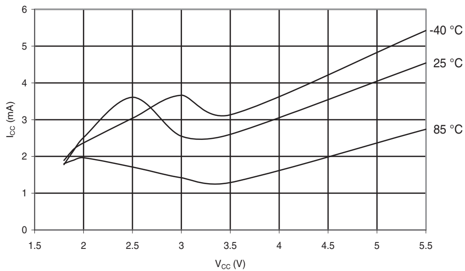
Figure 30-44. ATmega48A: Programming Current vs. V_{CC}
