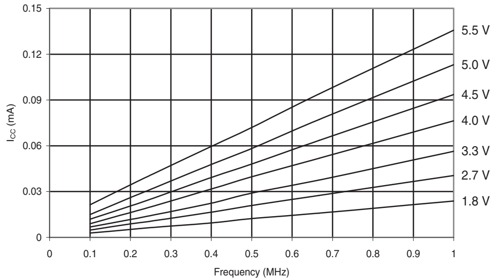
Figure 30-241. ATmega168PA: Idle Supply Current vs. Low Frequency (0.1-1.0MHz)
