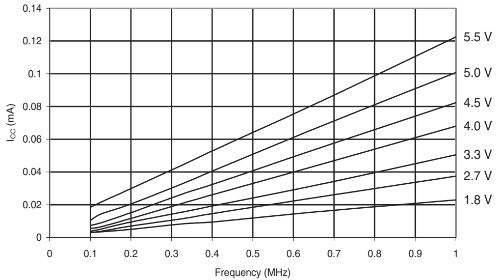
Figure 30-92. ATmega48PA: Reset Supply Current vs. Low Frequency (0.1 - 1.0MHz)
