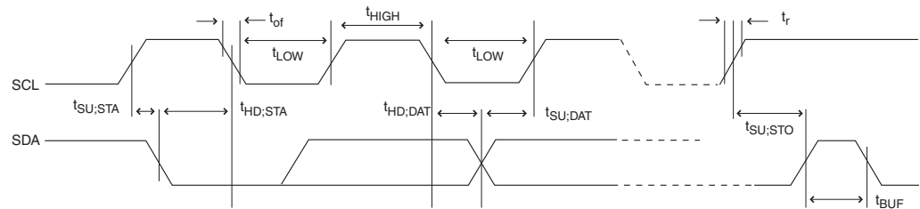
Figure 29-5. Two-wire Serial Bus Timing
