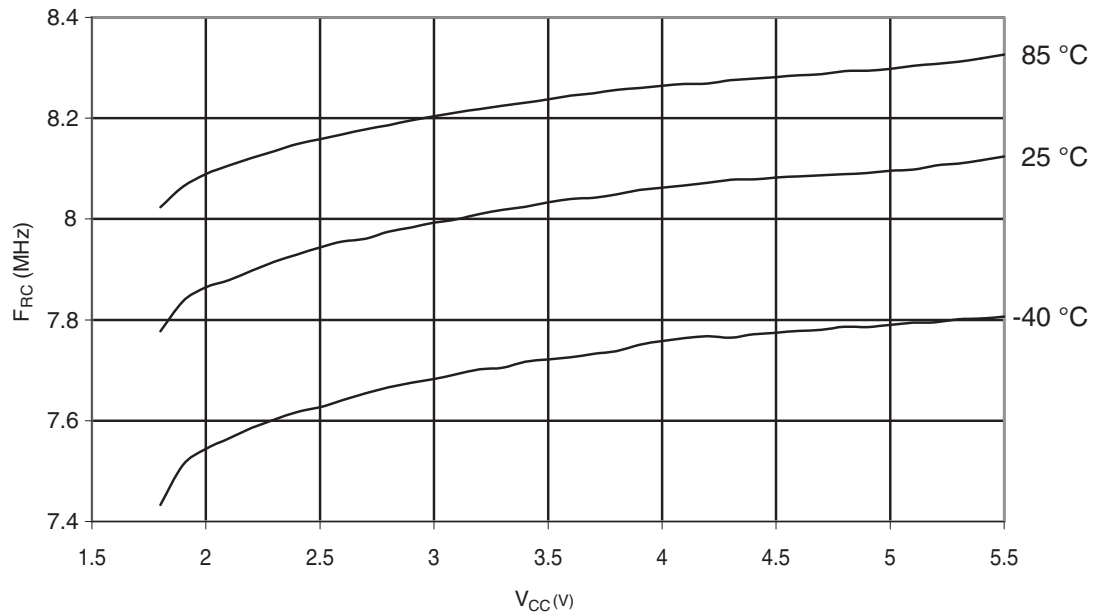
Figure 30-366. ATmega328P: Calibrated 8MHz RC Oscillator Frequency vs. V_{CC}
