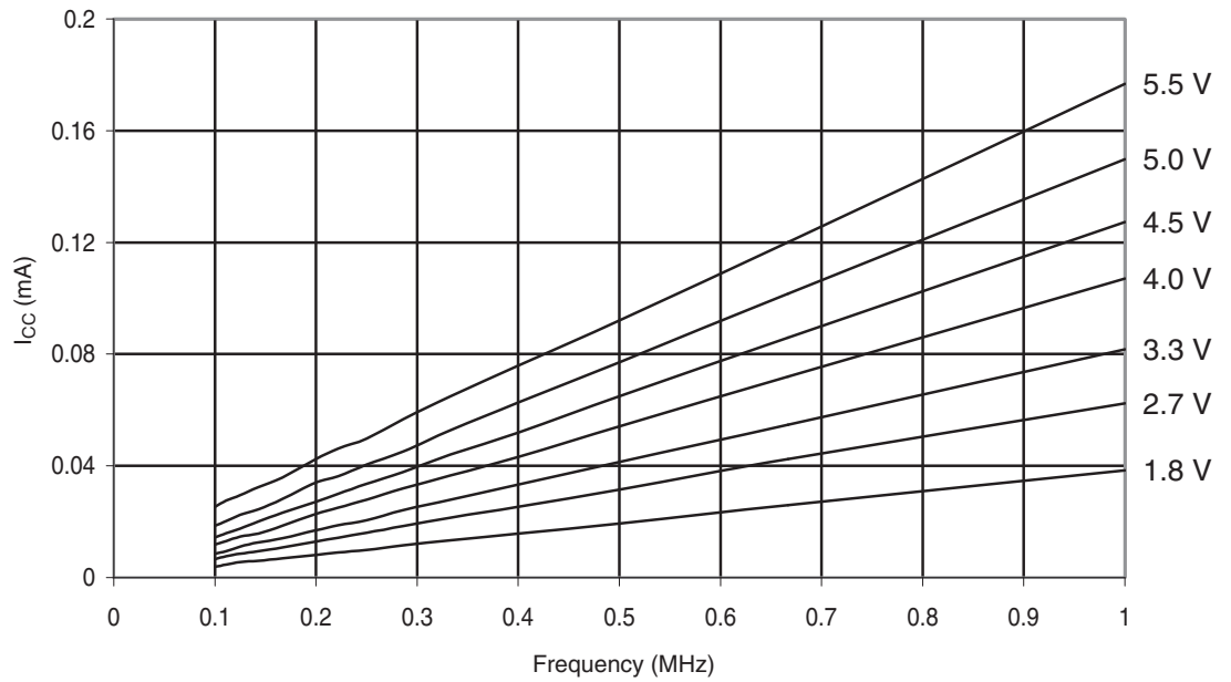
Figure 30-288. ATmega328: Idle Supply Current vs. Low Frequency (0.1-1.0MHz)
