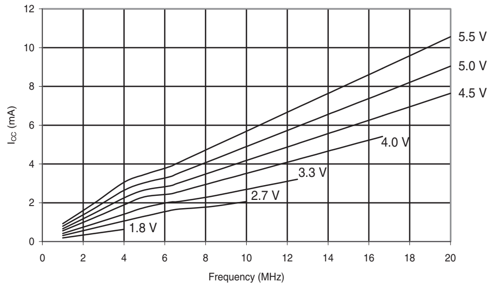
Figure 30-237. ATmega168PA: Active Supply Current vs. Frequency (1-20MHz)
