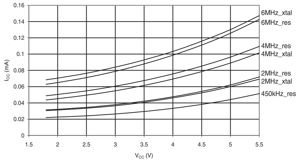
Figure 30-14. ATmega48A: Standby Supply Current vs. V_{CC} (Watchdog Timer Disabled)
