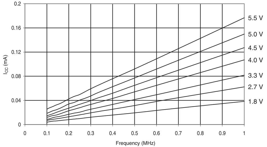
Figure 30-335. ATmega328P: Idle Supply Current vs. Low Frequency (0.1-1.0MHz)
