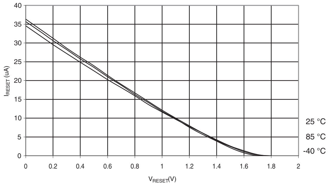
Figure 30-347. ATmega328P: Reset Pull-up Resistor Current vs. Reset Pin Voltage ( V_{CC} = 1.8\text{ V} )
