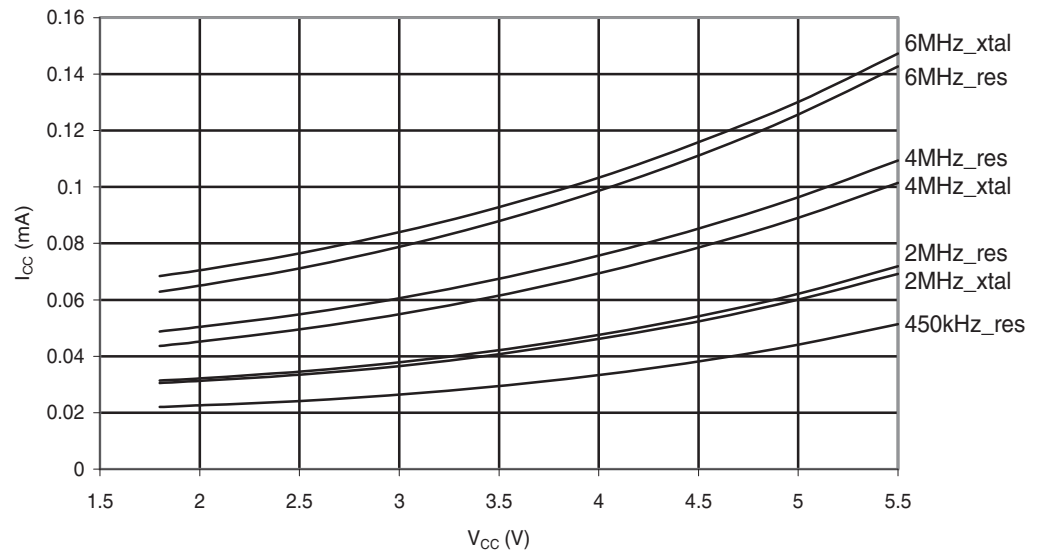
Figure 30-61. ATmega48PA: Standby Supply Current vs. V_{CC} (Watchdog Timer Disabled)
