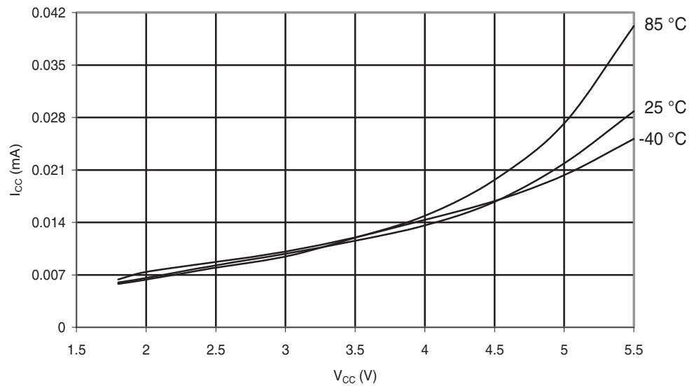
Figure 30-55. ATmega48PA: Idle Supply Current vs. V_{CC} (Internal RC Oscillator, 128kHz)
