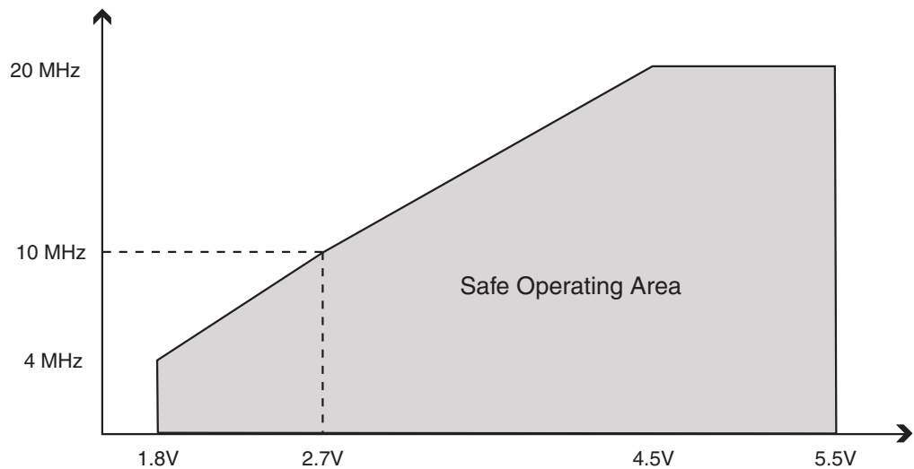
Figure 29-1. Maximum Frequency vs. V_{CC}
