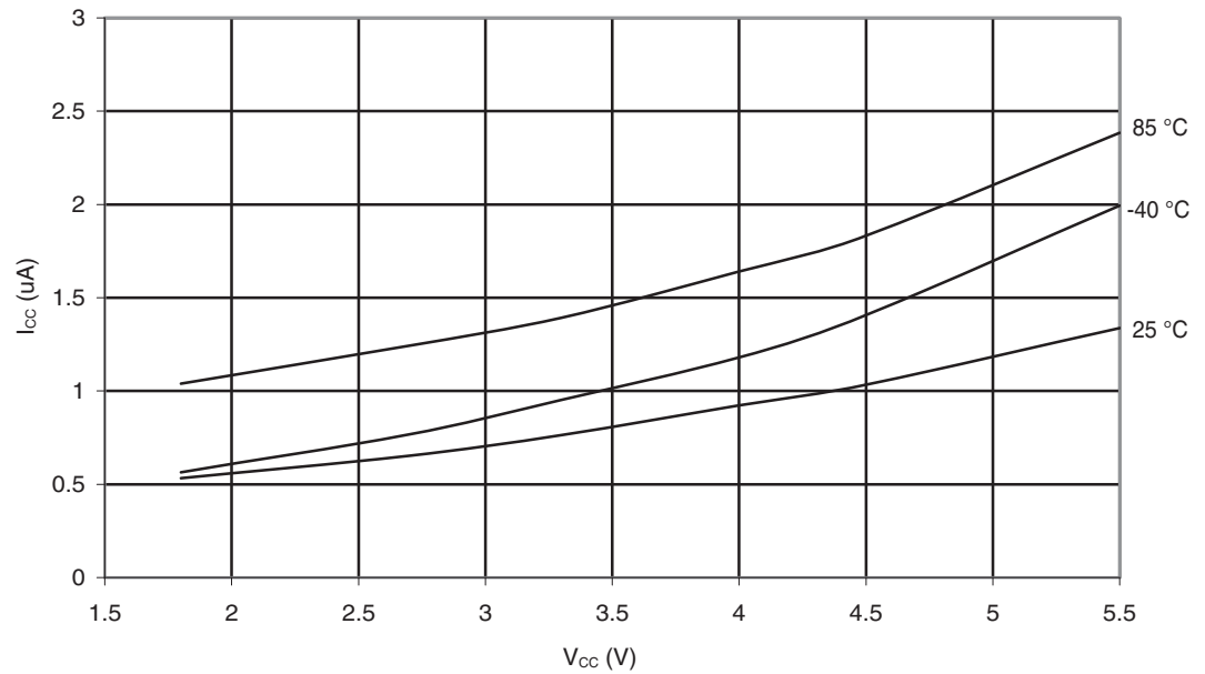
Figure 30-107. ATmega88A: Power-Save Supply Current vs. V_{CC} (Watchdog Timer Disabled and 32kHz Crystal Oscillator Running)
