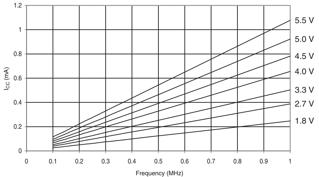
Figure 30-283. ATmega328: Active Supply Current vs. Low Frequency (0.1-1.0MHz)
