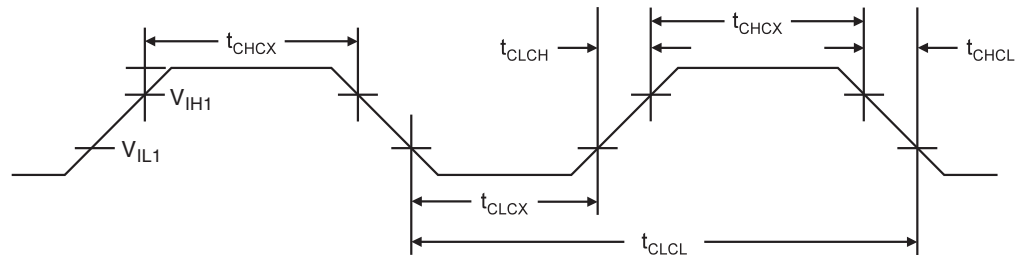
Figure 29-2. External Clock Drive Waveforms
