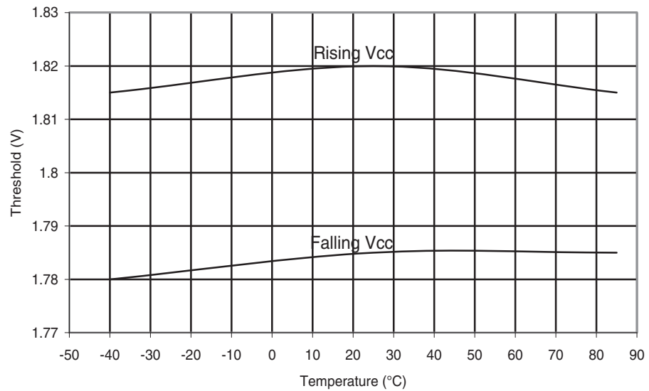
Figure 30-172. ATmega88PA: BOD Thresholds vs. Temperature (BODLEVEL is 1.8 V)
