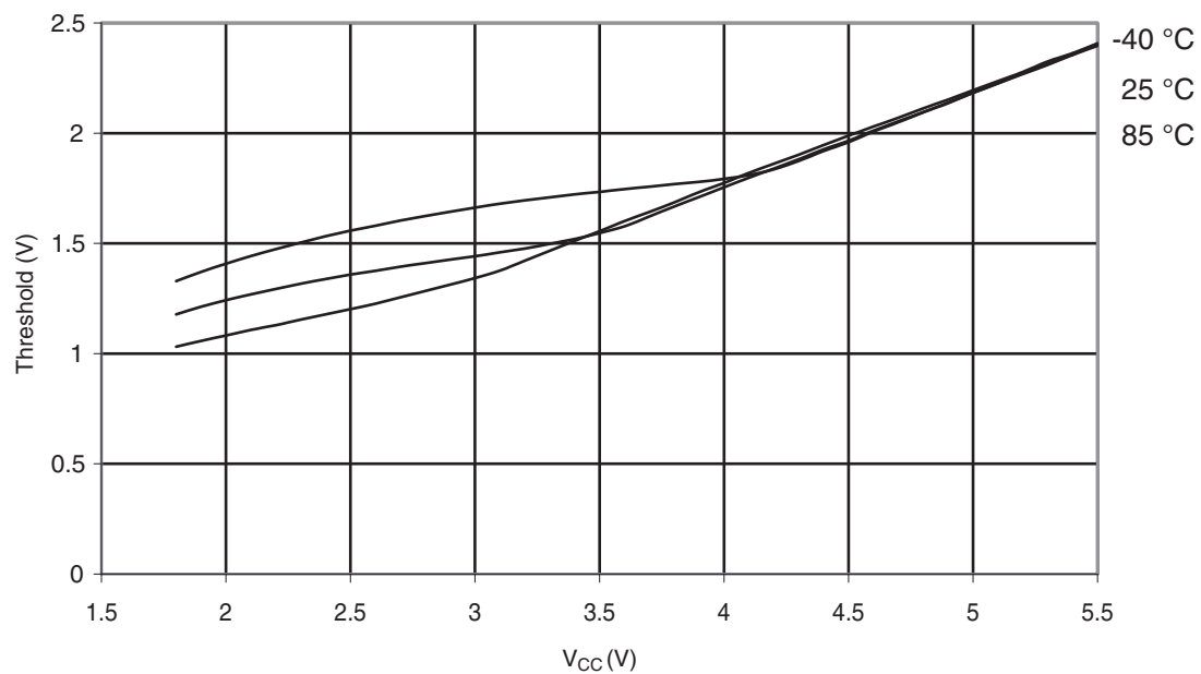
Figure 30-357. ATmega328P: Reset Input Threshold Voltage vs. V_{CC} ( V_{IH} , I/O Pin read as '1')
