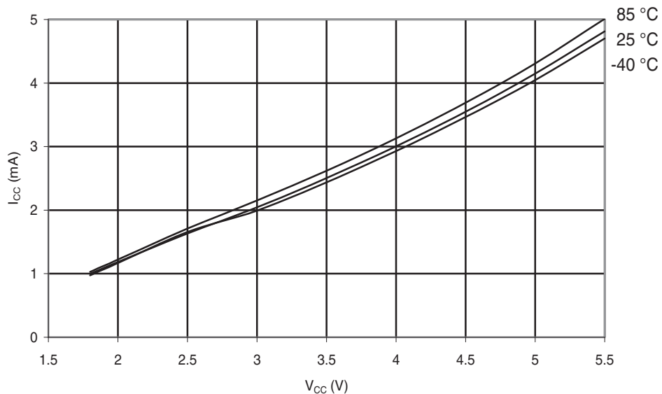
Figure 30-193. ATmega168A: Active Supply Current vs. V_{CC} (Internal RC Oscillator, 8MHz)
