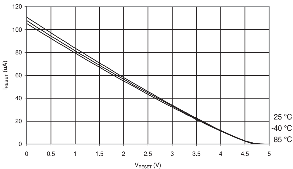
Figure 30-114. ATmega88A: Reset Pull-up Resistor Current vs. Reset Pin Voltage ( V_{CC} = 5\text{ V} )
