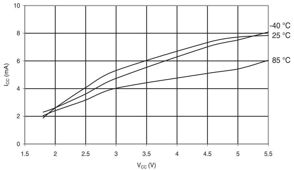
Figure 30-279. ATmega168PA: Programming Current vs. V_{CC}
