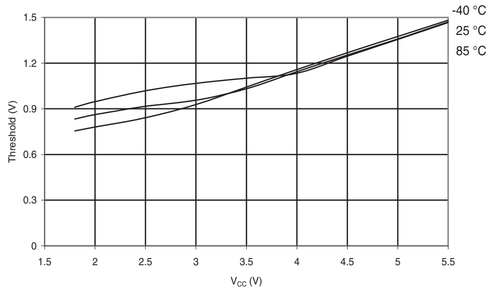
Figure 30-169. ATmega88PA: Reset Input Threshold Voltage vs. V_{CC} ( V_{IH} , I/O Pin read as '1')
