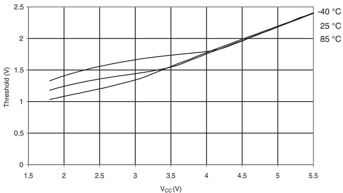
Figure 30-310. ATmega328: Reset Input Threshold Voltage vs. V_{CC} ( V_{IH} , I/O Pin read as '1')
