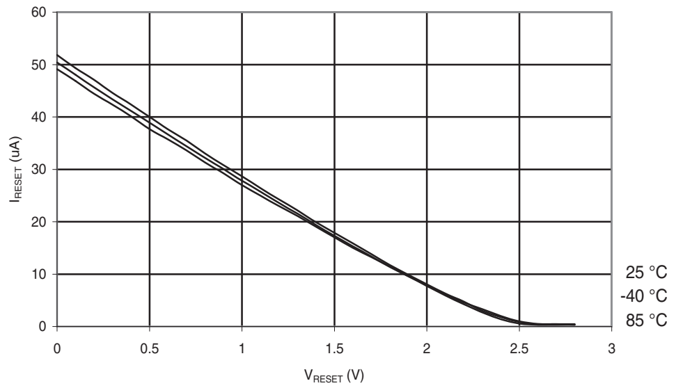
Figure 30-19. ATmega48A: Reset Pull-up Resistor Current vs. Reset Pin Voltage ( V_{CC} = 2.7\text{ V} )
