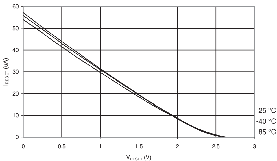
Figure 30-113. ATmega88A: Reset Pull-up Resistor Current vs. Reset Pin Voltage ( V_{CC} = 2.7\text{ V} )
