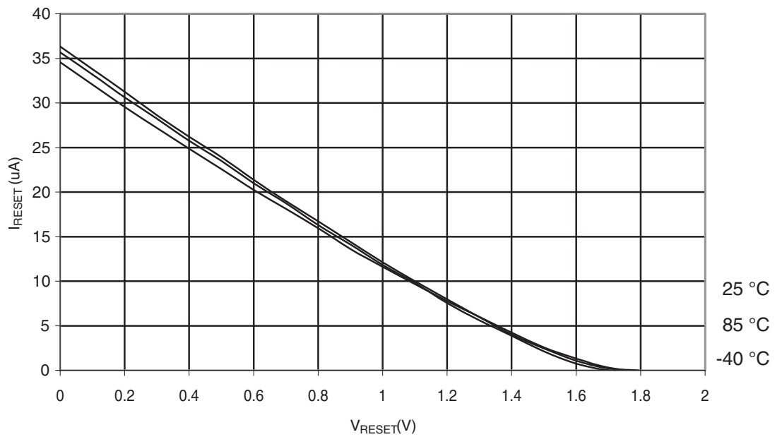
Figure 30-300. ATmega328: Reset Pull-up Resistor Current vs. Reset Pin Voltage ( V_{CC} = 1.8\text{ V} )
