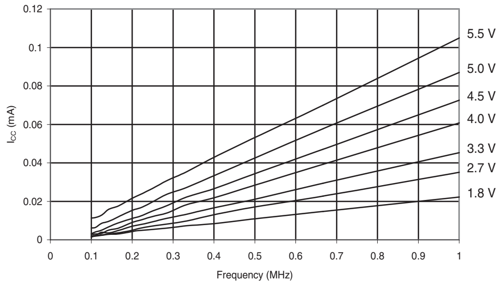
Figure 30-186. ATmega88PA: Reset Supply Current vs. Low Frequency (0.1 - 1.0MHz)
