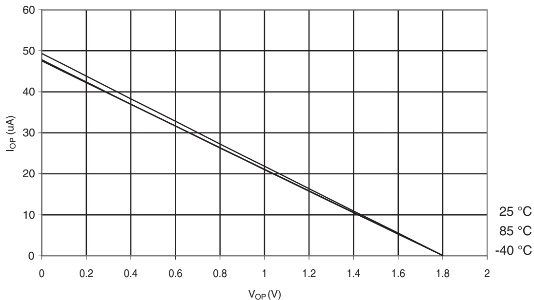
Figure 30-297. ATmega328: I/O Pin Pull-up Resistor Current vs. Input Voltage ( V_{CC} = 1.8\text{ V} )
