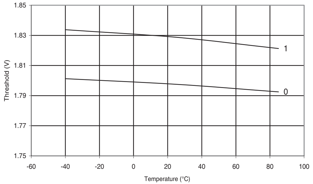
Figure 30-360. ATmega328P: BOD Thresholds vs. Temperature (BODLEVEL is 1.8 V)
