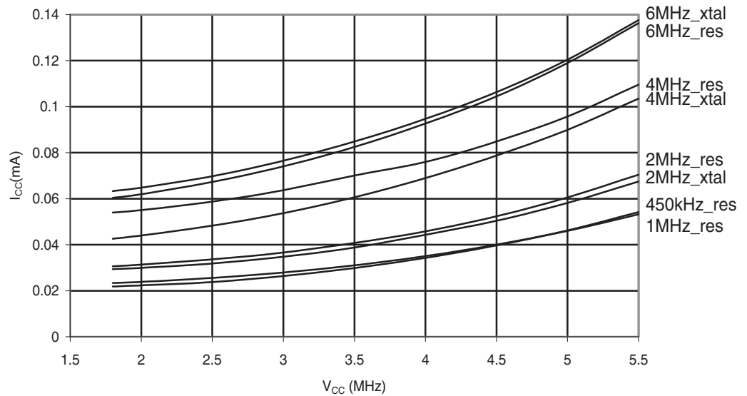
Figure 30-202. ATmega168A: Standby Supply Current vs. V_{CC} (Watchdog Timer Disabled)
