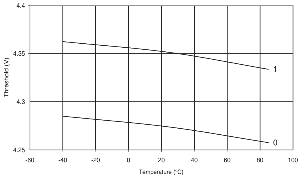
Figure 30-362. ATmega328P: BOD Thresholds vs. Temperature (BODLEVEL is 4.3 V)
