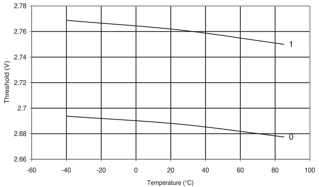
Figure 30-361. ATmega328P: BOD Thresholds vs. Temperature (BODLEVEL is 2.7 V)
