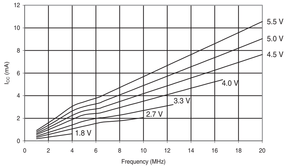
Figure 30-190. ATmega168A: Active Supply Current vs. Frequency (1-20MHz)
