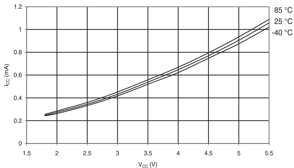
Figure 30-192. ATmega168A: Active Supply Current vs. V_{CC} (Internal RC Oscillator, 1MHz)
