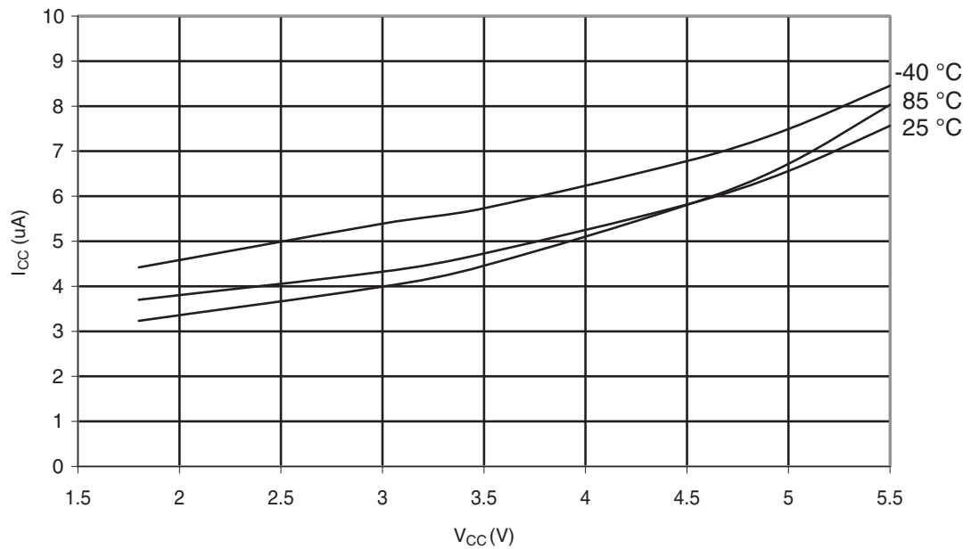
Figure 30-294. ATmega328: Power-Down Supply Current vs. V_{CC} (Watchdog Timer Enabled)
