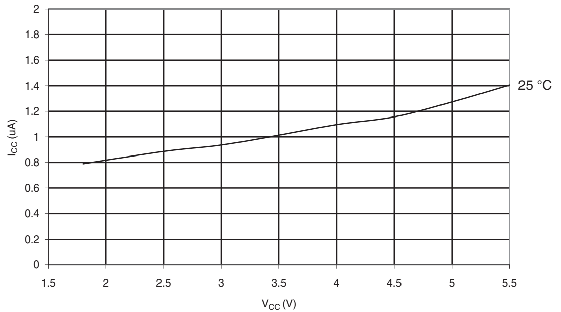
Figure 30-295. ATmega328: Power-Save Supply Current vs. V_{CC} (Watchdog Timer Disabled and 32kHz Crystal Oscillator Running)
