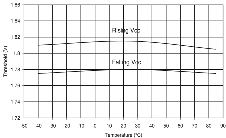
Figure 30-266. ATmega168PA: BOD Thresholds vs. Temperature (BODLEVEL is 1.8 V)
