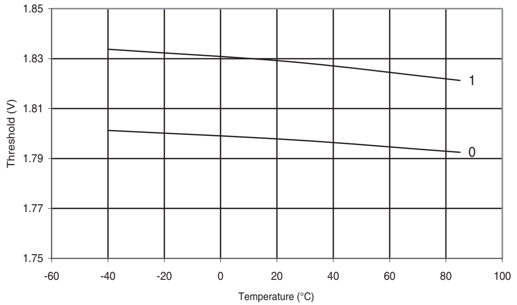
Figure 30-313. ATmega328: BOD Thresholds vs. Temperature (BODLEVEL is 1.8 V)
