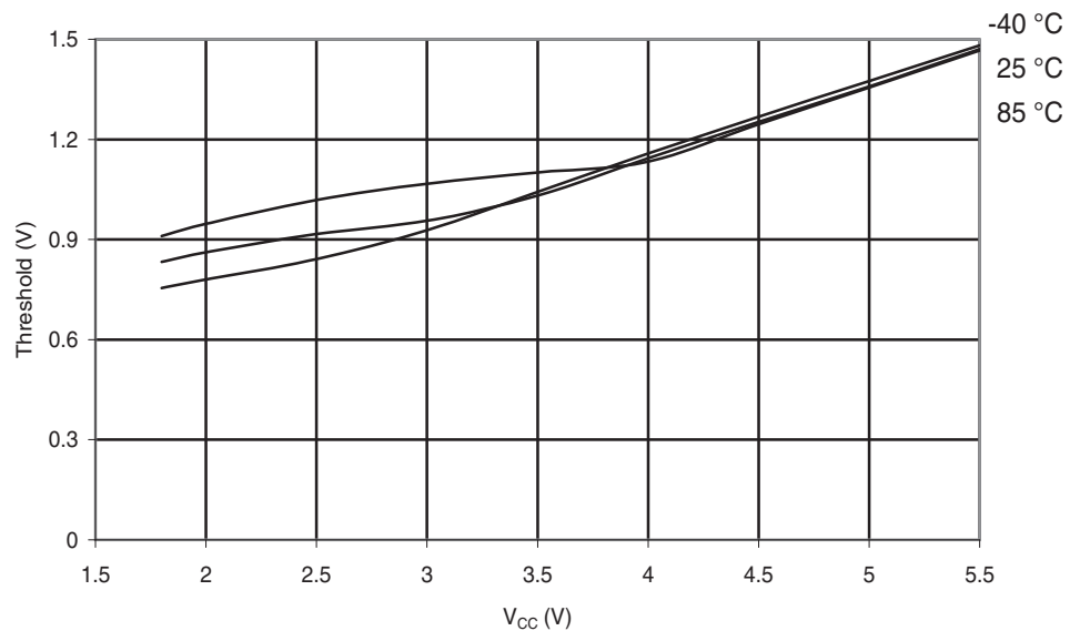
Figure 30-122. ATmega88A: Reset Input Threshold Voltage vs. V_{CC} ( V_{IH} , I/O Pin read as '1')
