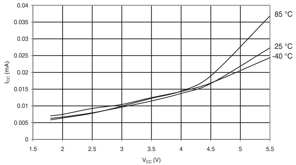
Figure 30-243. ATmega168PA: Idle Supply Current vs. V_{CC} (Internal RC Oscillator, 128kHz)
