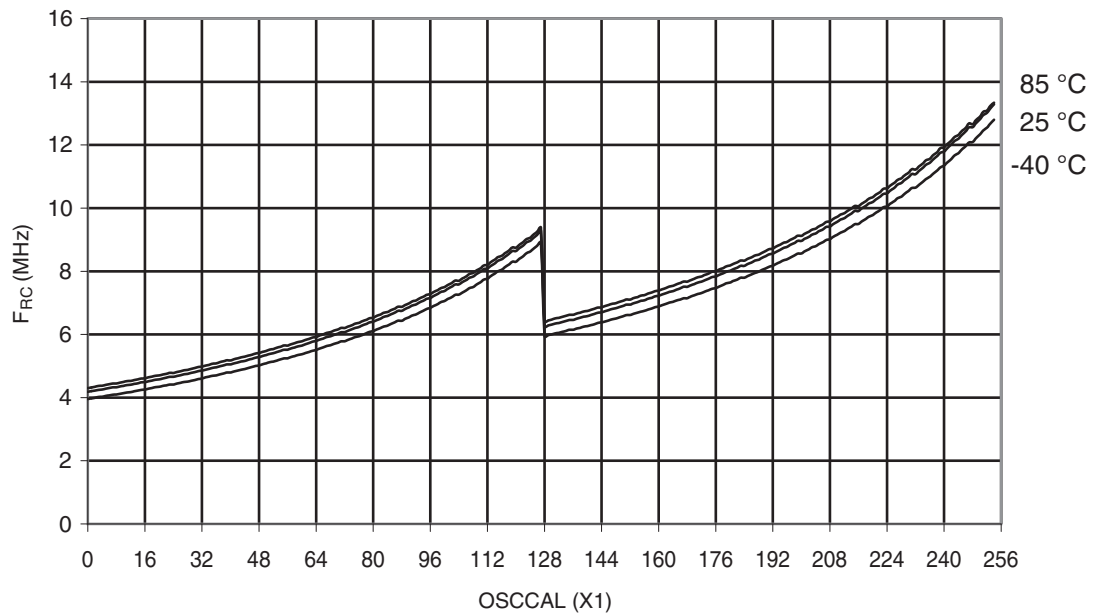
Figure 30-321. ATmega328: Calibrated 8MHz RC Oscillator Frequency vs. OSCCAL Value
