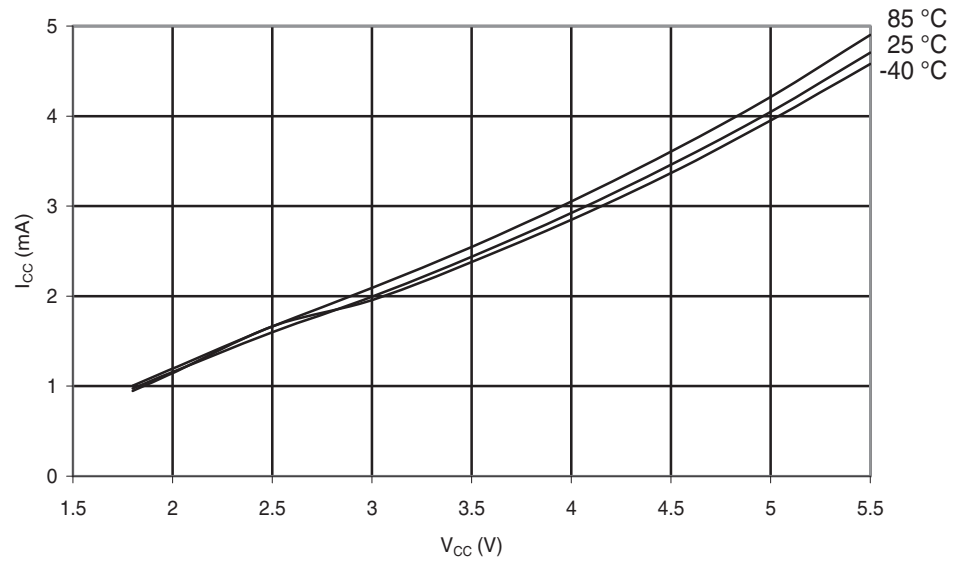
Figure 30-52. ATmega48PA: Active Supply Current vs. V_{CC} (Internal RC Oscillator, 8MHz)
