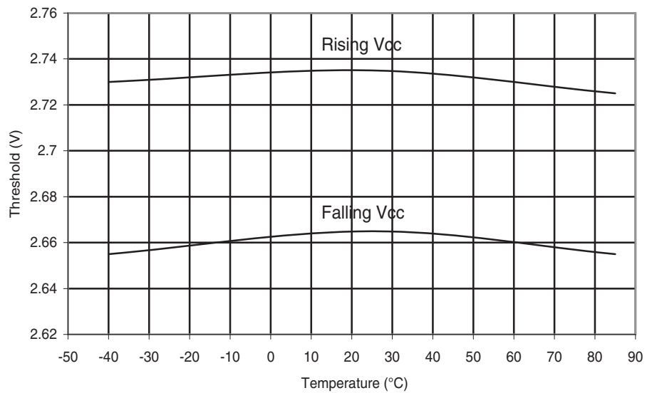
Figure 30-220. ATmega168A: BOD Thresholds vs. Temperature (BODLEVEL is 2.7 V)
