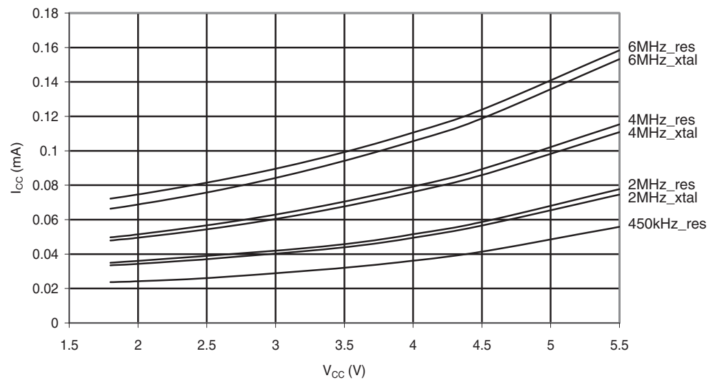
Figure 30-155. ATmega88PA: Standby Supply Current vs. V_{CC} (Watchdog Timer Disabled)
