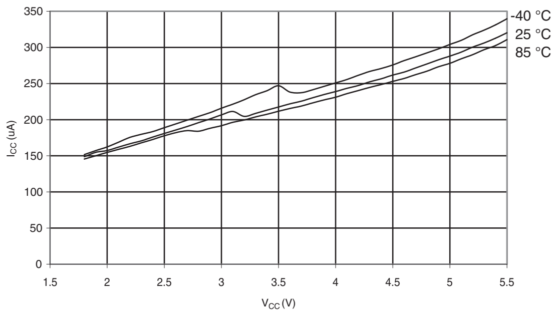
Figure 30-369. ATmega328P: ADC Current vs. V_{CC} (AREF = AV_{CC} )
