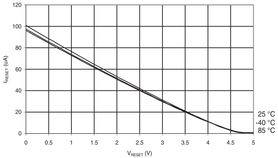
Figure 30-20. ATmega48A: Reset Pull-up Resistor Current vs. Reset Pin Voltage ( V_{CC} = 5\text{ V} )
