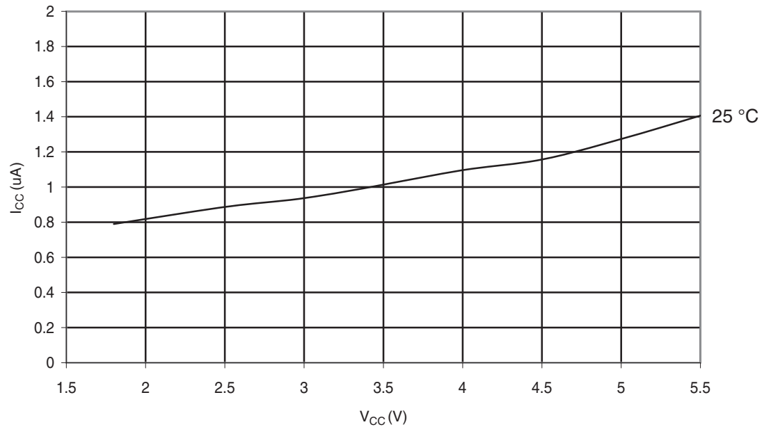
Figure 30-342. ATmega328P: Power-Save Supply Current vs. V_{CC} (Watchdog Timer Disabled and 32kHz Crystal Oscillator Running)
