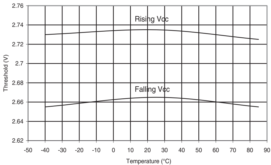
Figure 30-267. ATmega168PA: BOD Thresholds vs. Temperature (BODLEVEL is 2.7 V)
