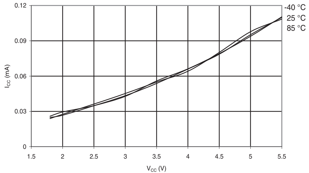
Figure 30-144. ATmega88PA: Active Supply Current vs. V_{CC} (Internal RC Oscillator, 128kHz)
