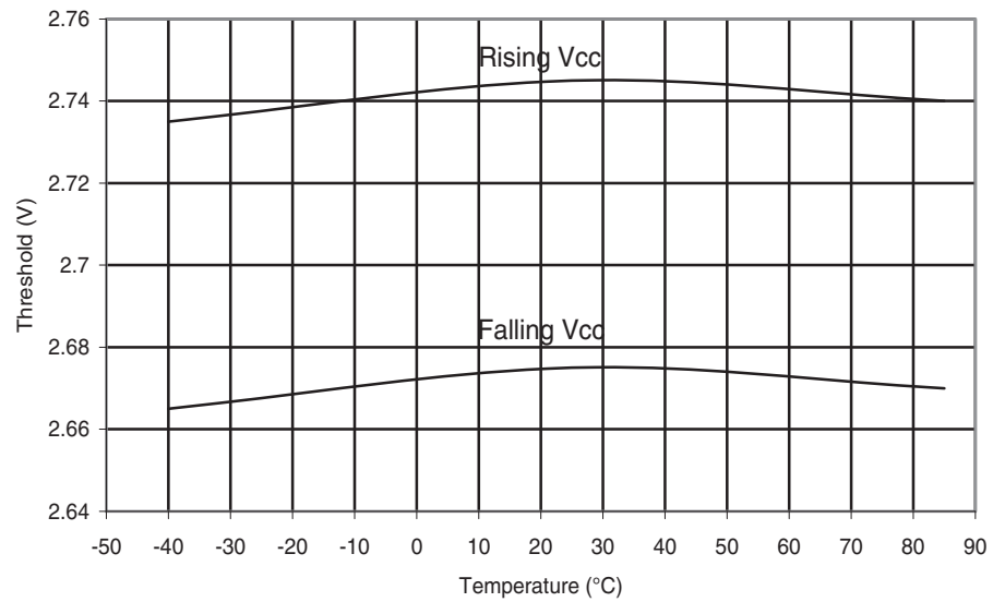
Figure 30-126. ATmega88A: BOD Thresholds vs. Temperature (BODLEVEL is 2.7 V)
