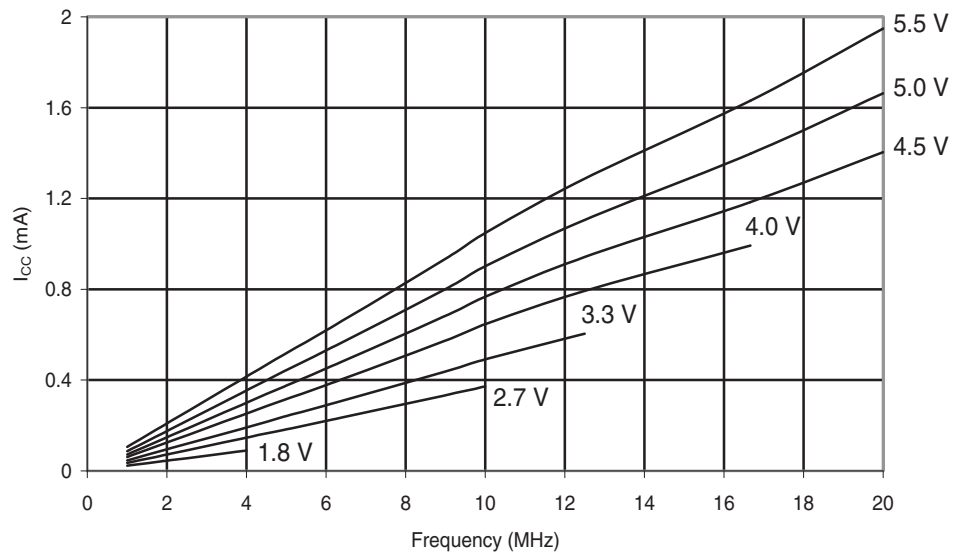
Figure 30-140. ATmega88A: Reset Supply Current vs. Frequency (1 - 20MHz)
