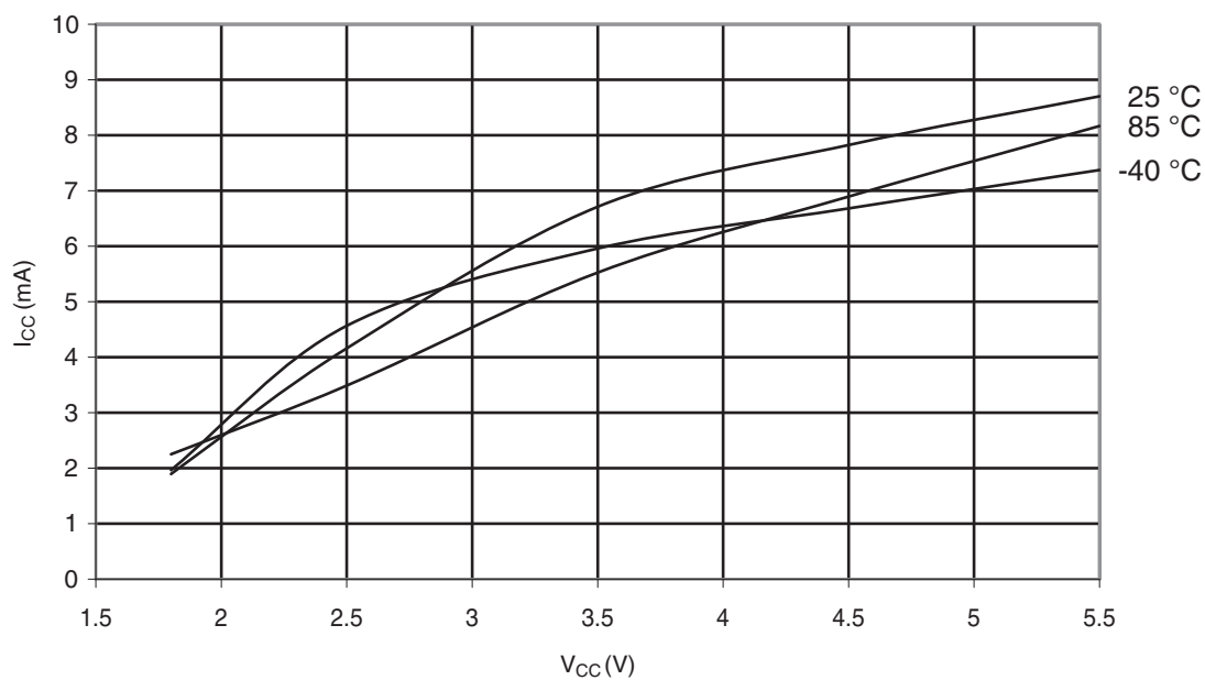
Figure 30-326. ATmega328: Programming Current vs. V_{CC}
