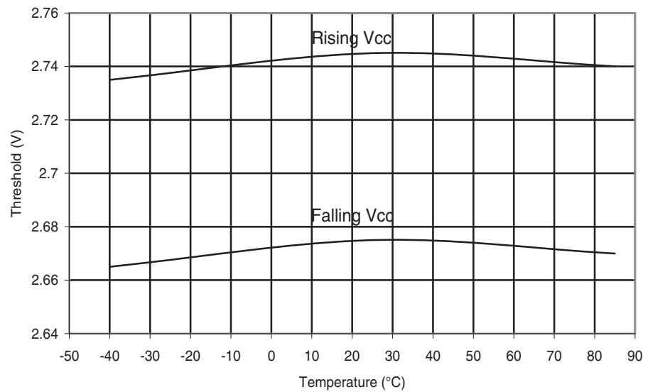
Figure 30-173. ATmega88PA: BOD Thresholds vs. Temperature (BODLEVEL is 2.7 V)
