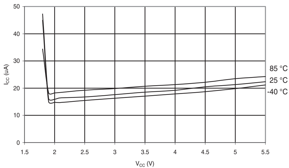
Figure 30-184. ATmega88PA: Brownout Detector Current vs. V_{CC}
