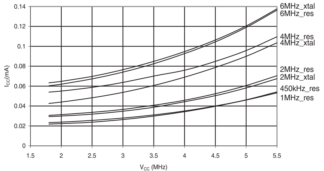
Figure 30-249. ATmega168PA: Standby Supply Current vs. V_{CC} (Watchdog Timer Disabled)
