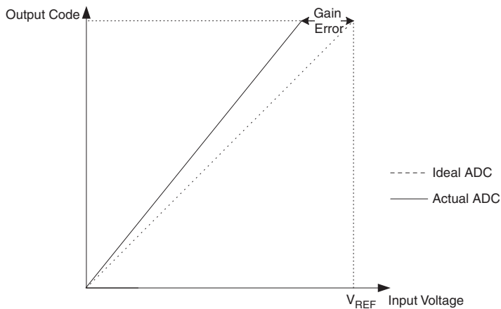
Figure 24-11. Gain Error
