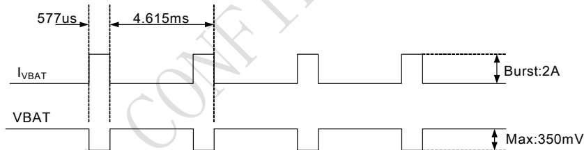
Figure 8: VBAT voltage drop during transmit burst
