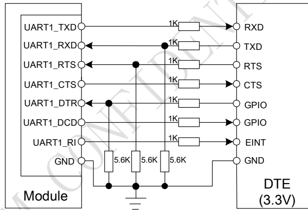
Figure 19: Resistor matching circuit
