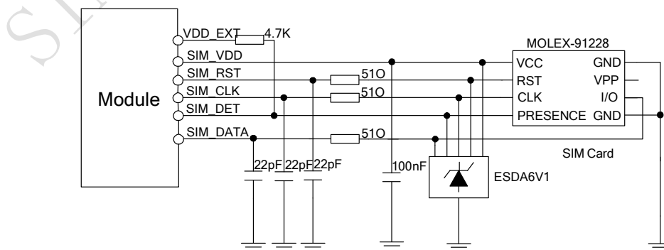
Figure 30: Reference circuit of the 8-pin SIM card holder
