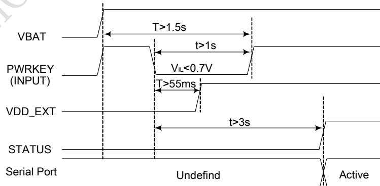
Figure 12: Timing of power on module
