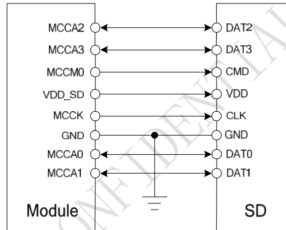
Figure 34: SD reference circuit
