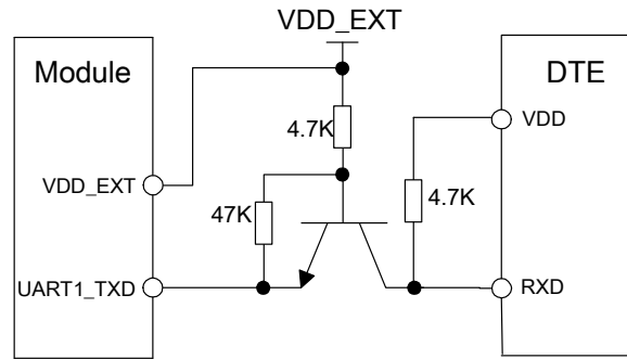
Figure 21: TX level matching circuit
