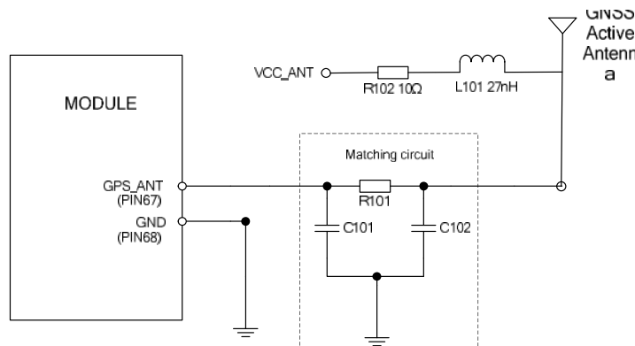
Figure 40: GNSS active antenna matching circuit
