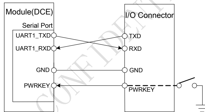
Figure 24: Connection for software upgrading and debugging
