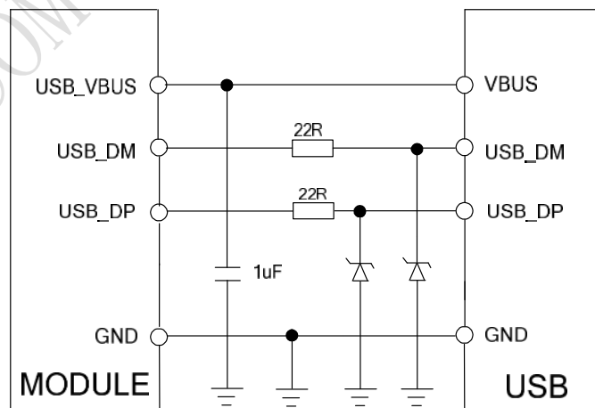
Figure 23: USB reference circuit
