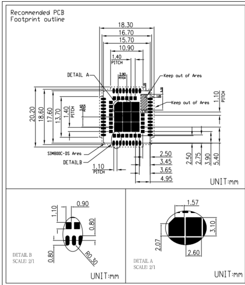
Figure 4: Recommended PCB footprint outline (Unit: mm)
