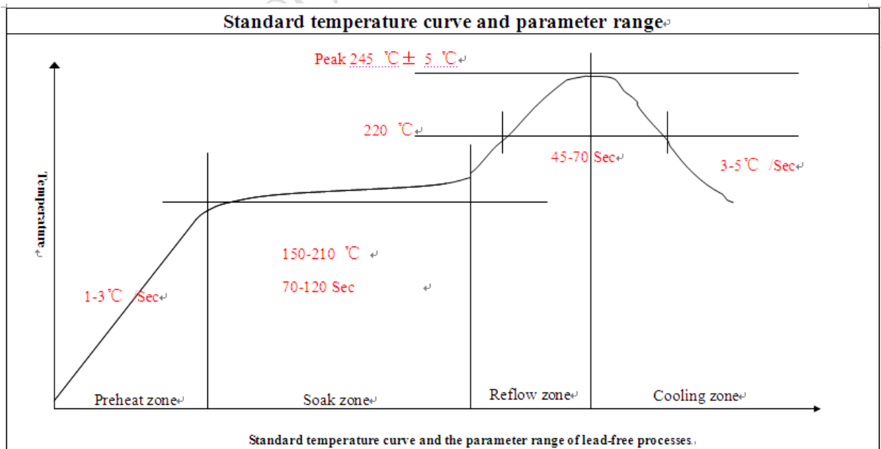
Figure 43: Typical solder reflow profile of lead-free process
