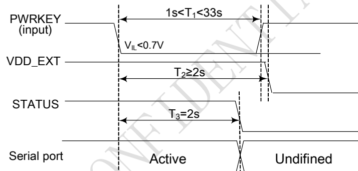
Figure 13: Timing of power off SIM868 by PWRKEY
