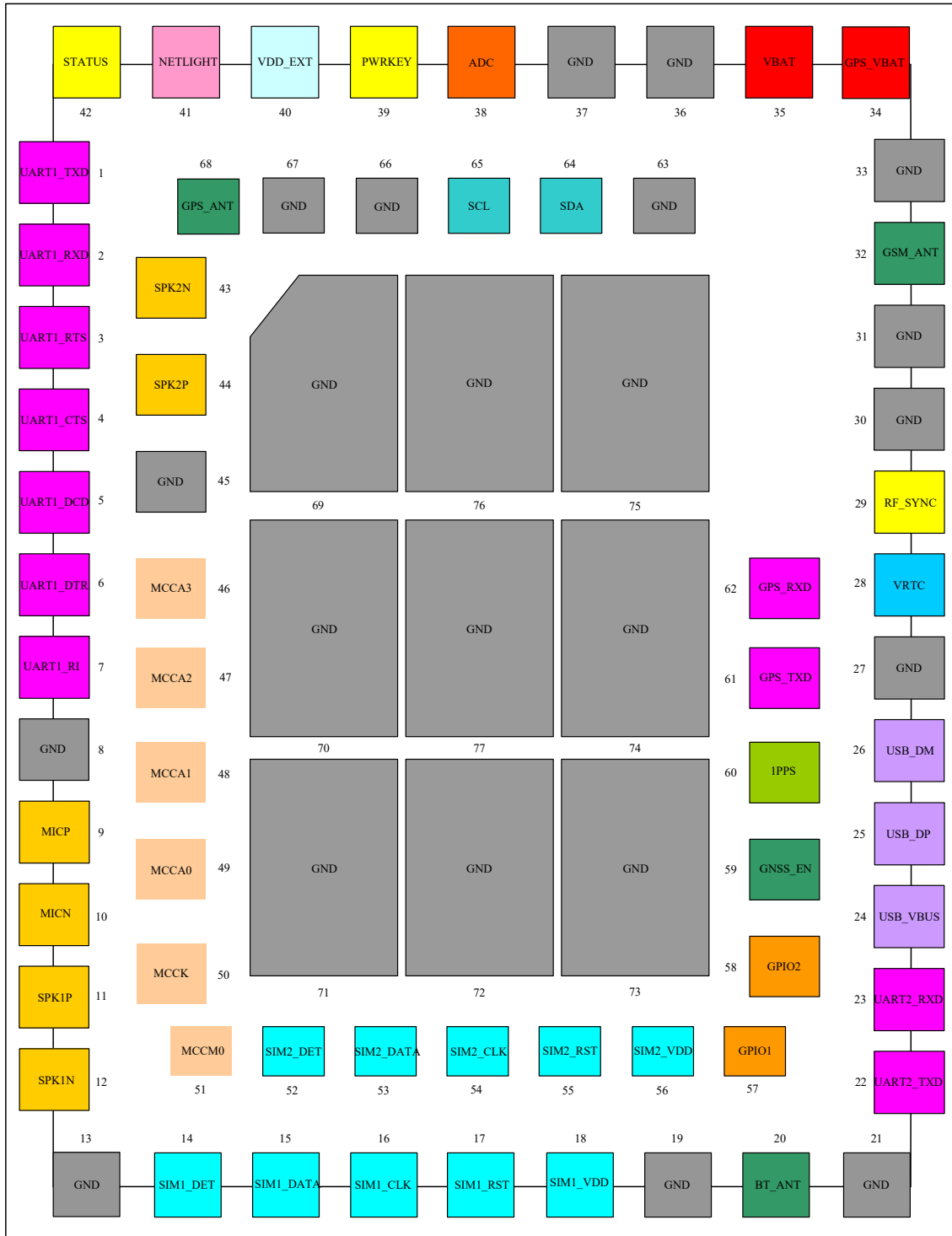
Figure 41: PIN assignment
