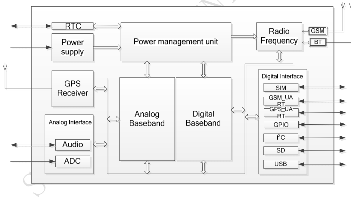
Figure 1: SIM868 functional diagram
