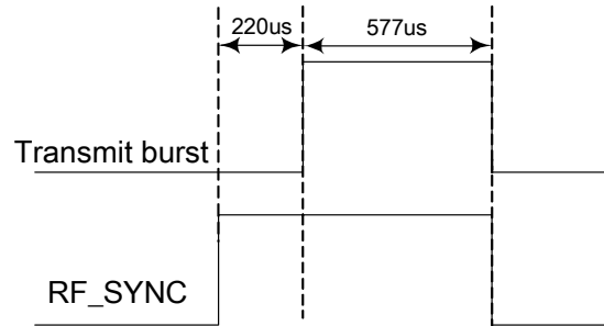
Figure 36: RF_SYNC signal during transmit burst
