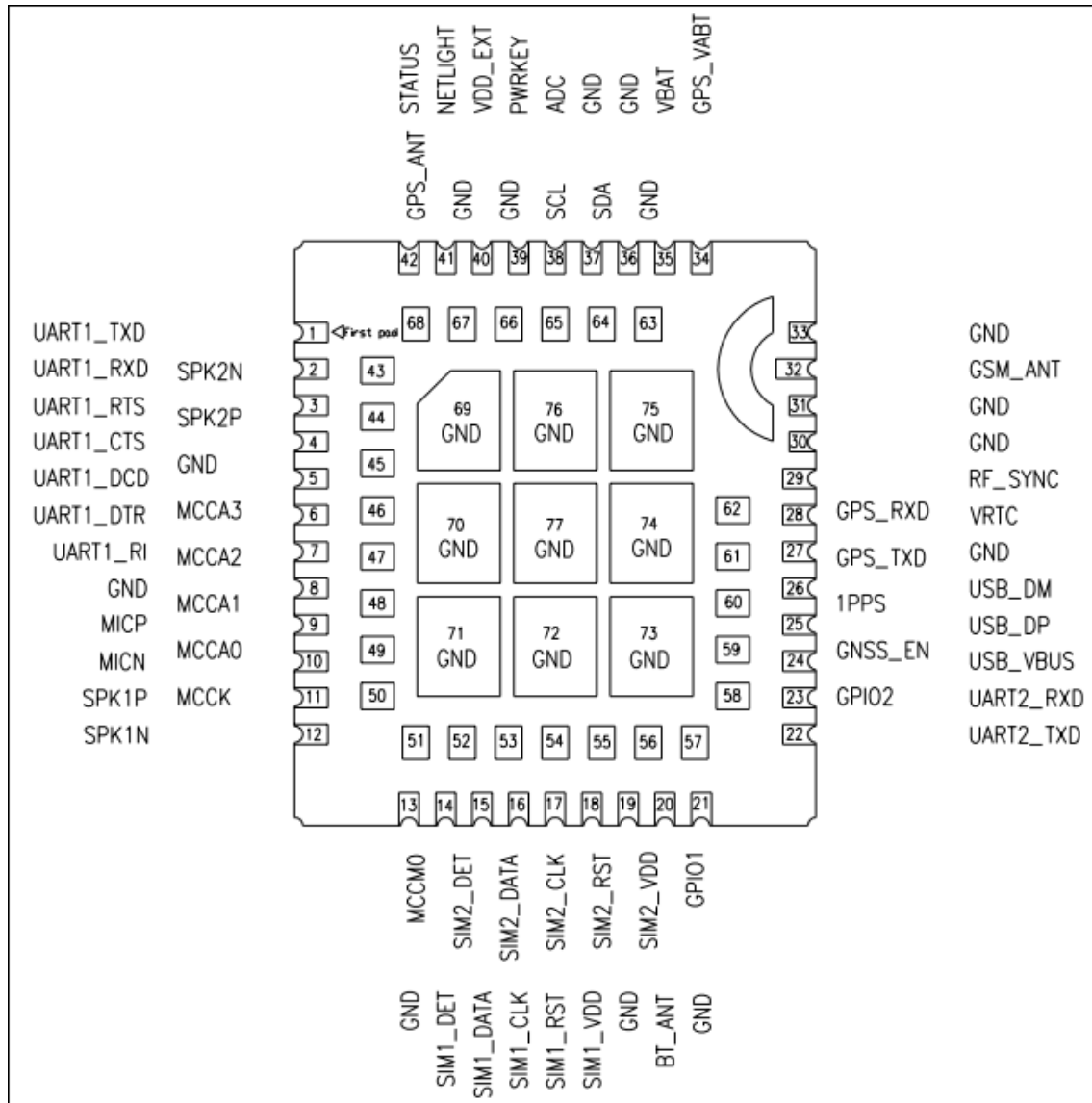
Figure 2: Pin out Diagram (Top view)
