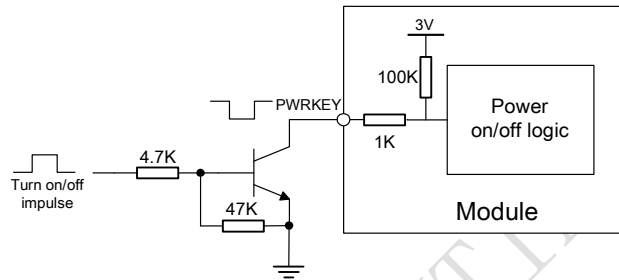
Figure 10: Powered on/down module using transistor
