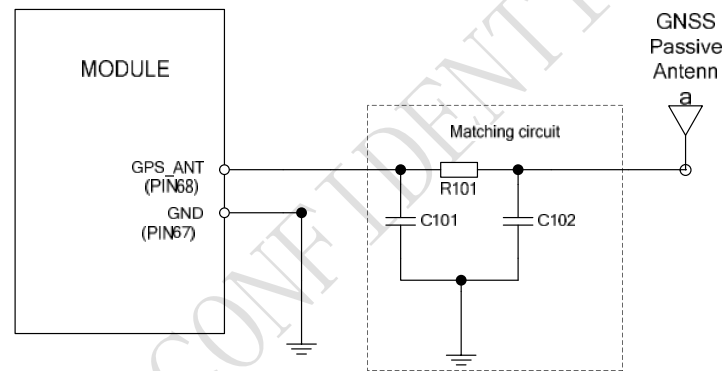
Figure 39: GNSS passive antenna matching circuit
