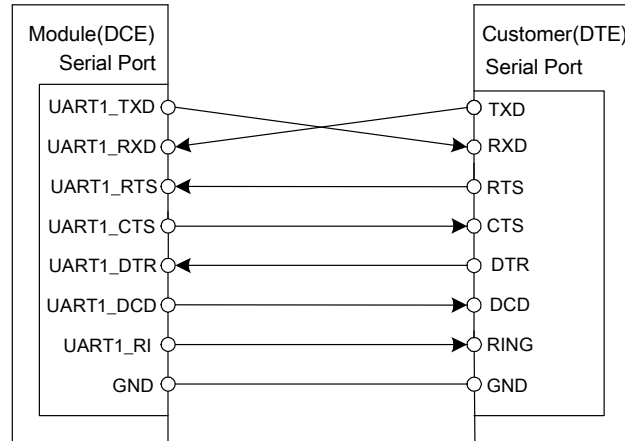
Figure 18: Connection of the serial interfaces
