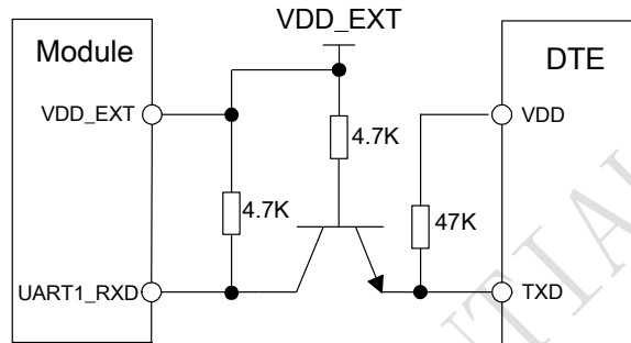
Figure 22: RX level matching circuit
