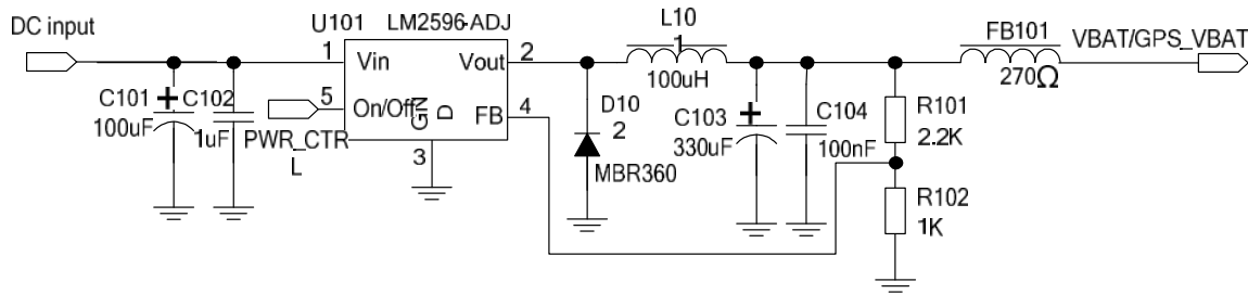
Figure 7: Reference circuit of the DC-DC power supply
