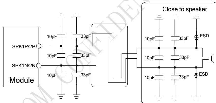
Figure 28: Speaker reference circuit
