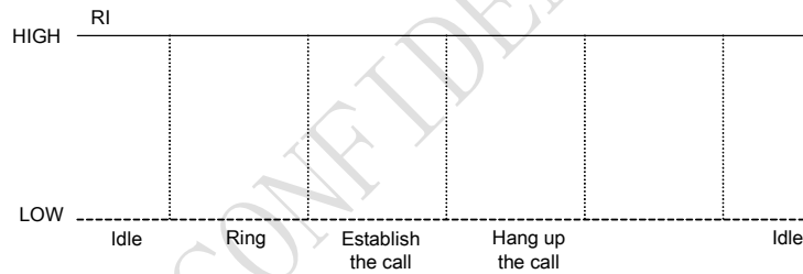
Figure 27: UART1_RI behaviour as a caller
