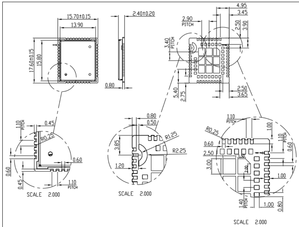
Figure 3: Dimensions of SIM868 (Unit: mm)
