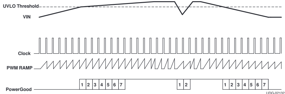
Figure 7-2. Undervoltage Lockout Operation
