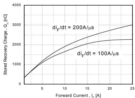
Figure 20. Stored Charge
