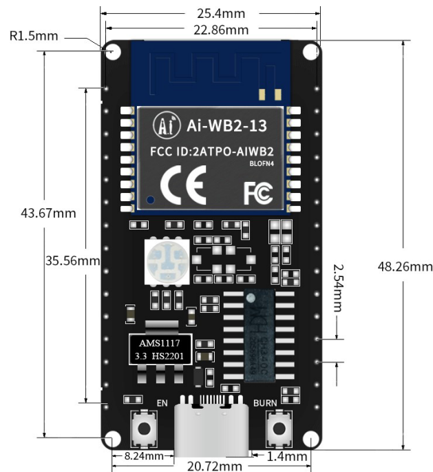
Figure 4 size chart
