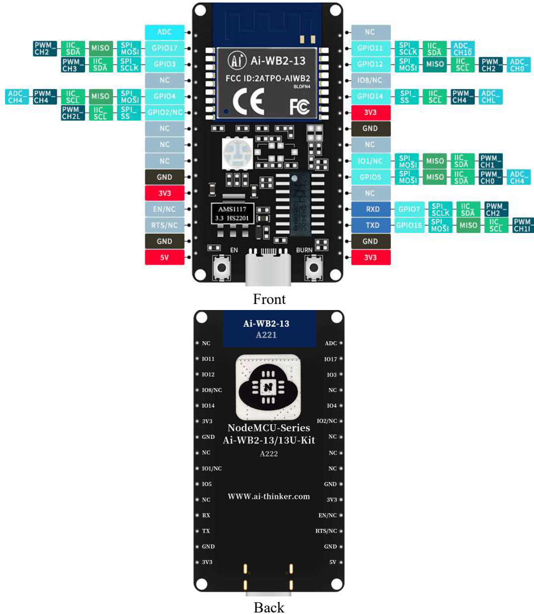
Figure 5 pin diagram
