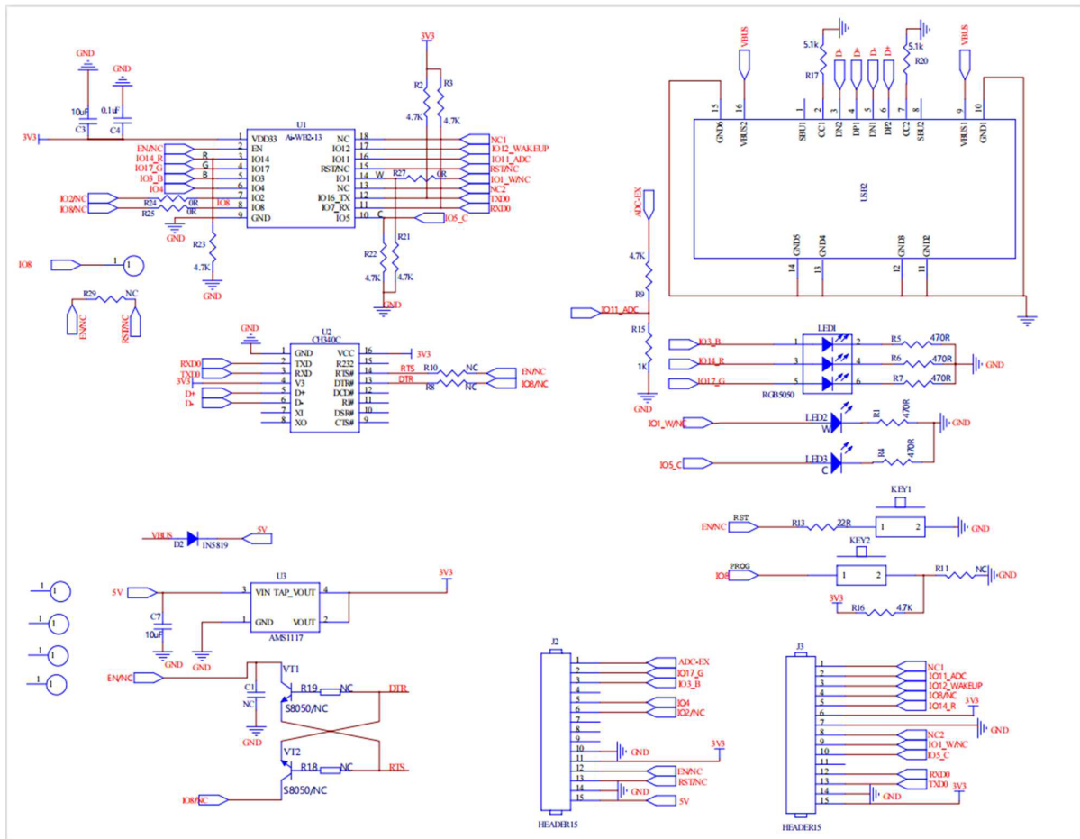
Figure 6 schematic diagram
