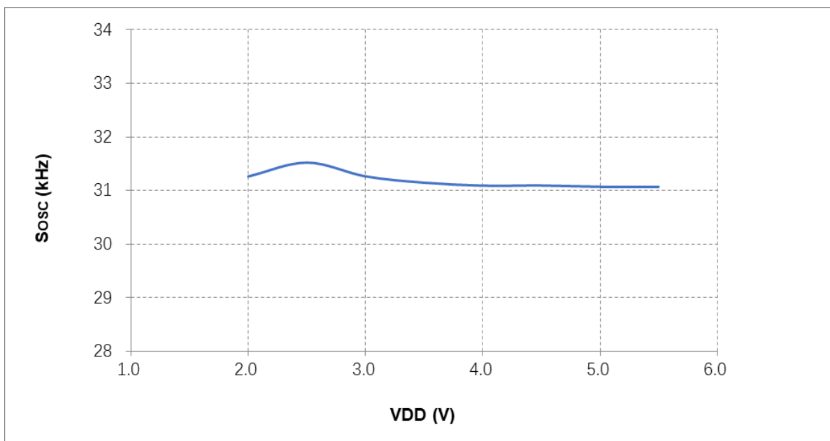
图 19-2 LIRC vs. V_{DD} ( T_A = 25^\circ\text{C} )
