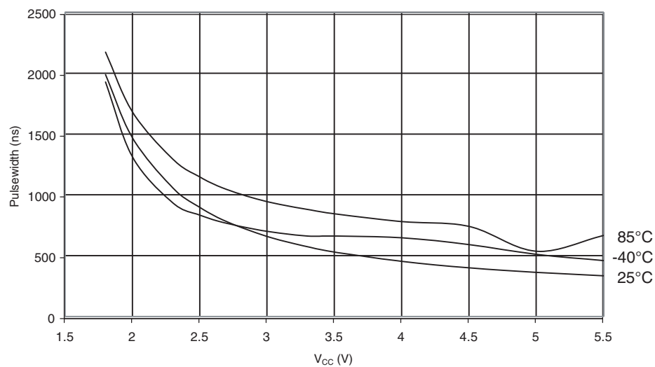
Figure 30-51. Reset pulse width vs. V_{CC} .
