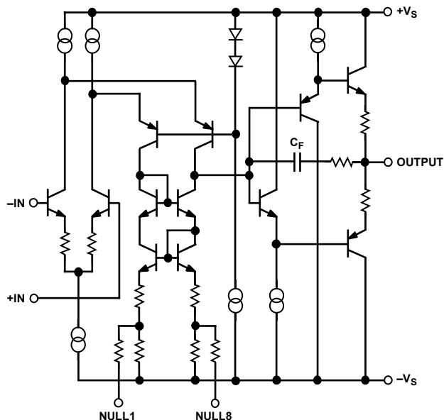
Figure 35. Simplified Schematic
