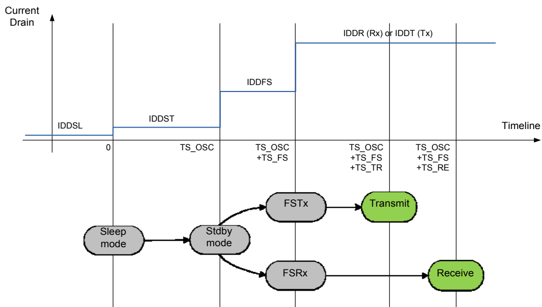
Figure 17. Startup Process
