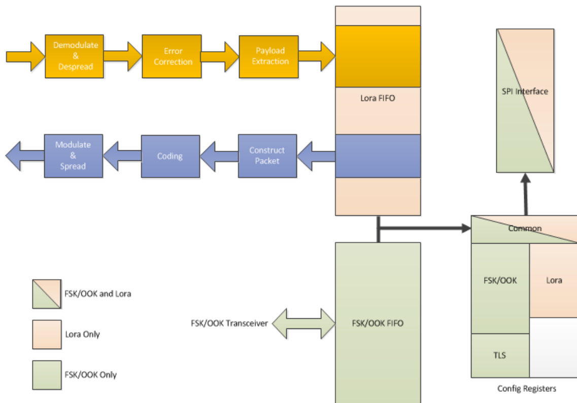
Figure 4. LoRa TM Modem Connectivity
