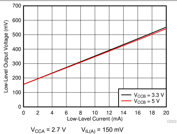
Figure 6-2. Low-Level Output Voltage ( V_{OL(Ax)} ) vs Low-Level Current ( I_{OL(Ax)} )
