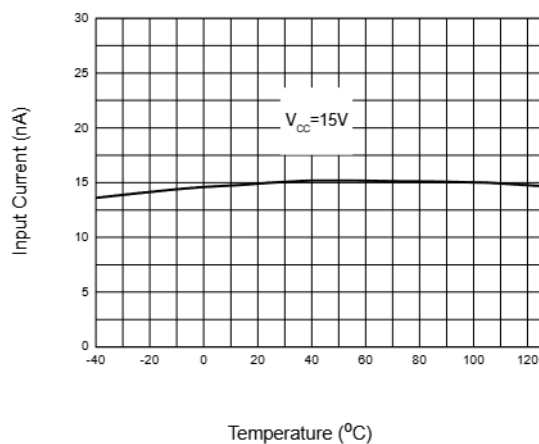
Figure 5. Input Current
