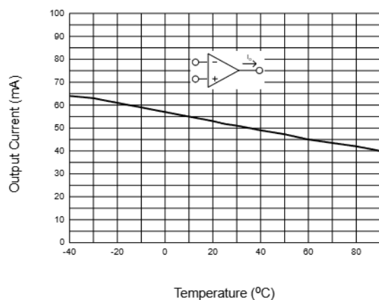
Figure 14. Current Limiting
