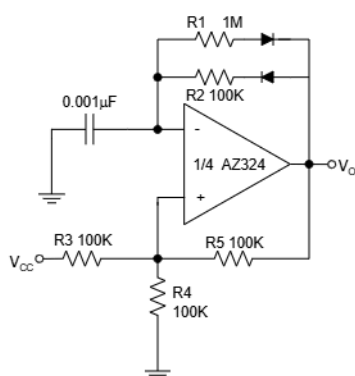
Figure 20. Pulse Generator
