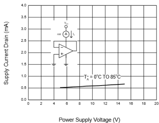
Figure 6. Supply Current
